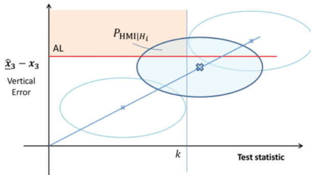
Figure 3. Representation of the weighted RAIM's V_{\text{slope}} concept.
