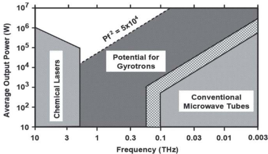
Figure 1. Domain of microwave tubes/ laser devices.
