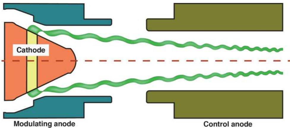
Figure 8. Cut-section view of a typical MIG.
