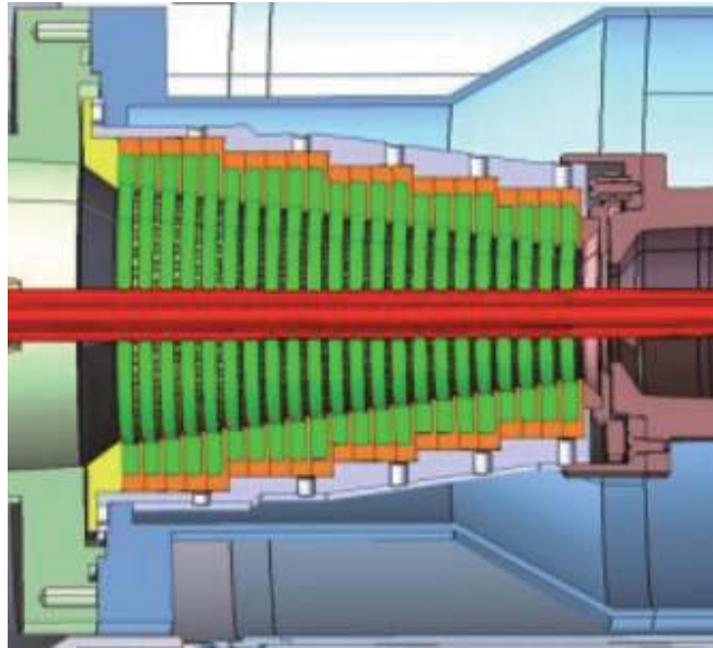
Figure 10. Cut section view of a beam tunnel.
