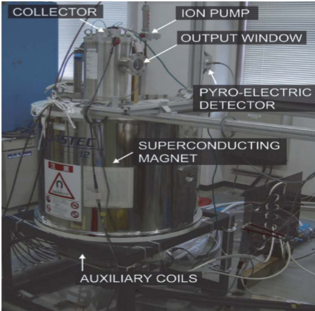
Figure 14. 2 MW Gyrotron for ECRH application.
