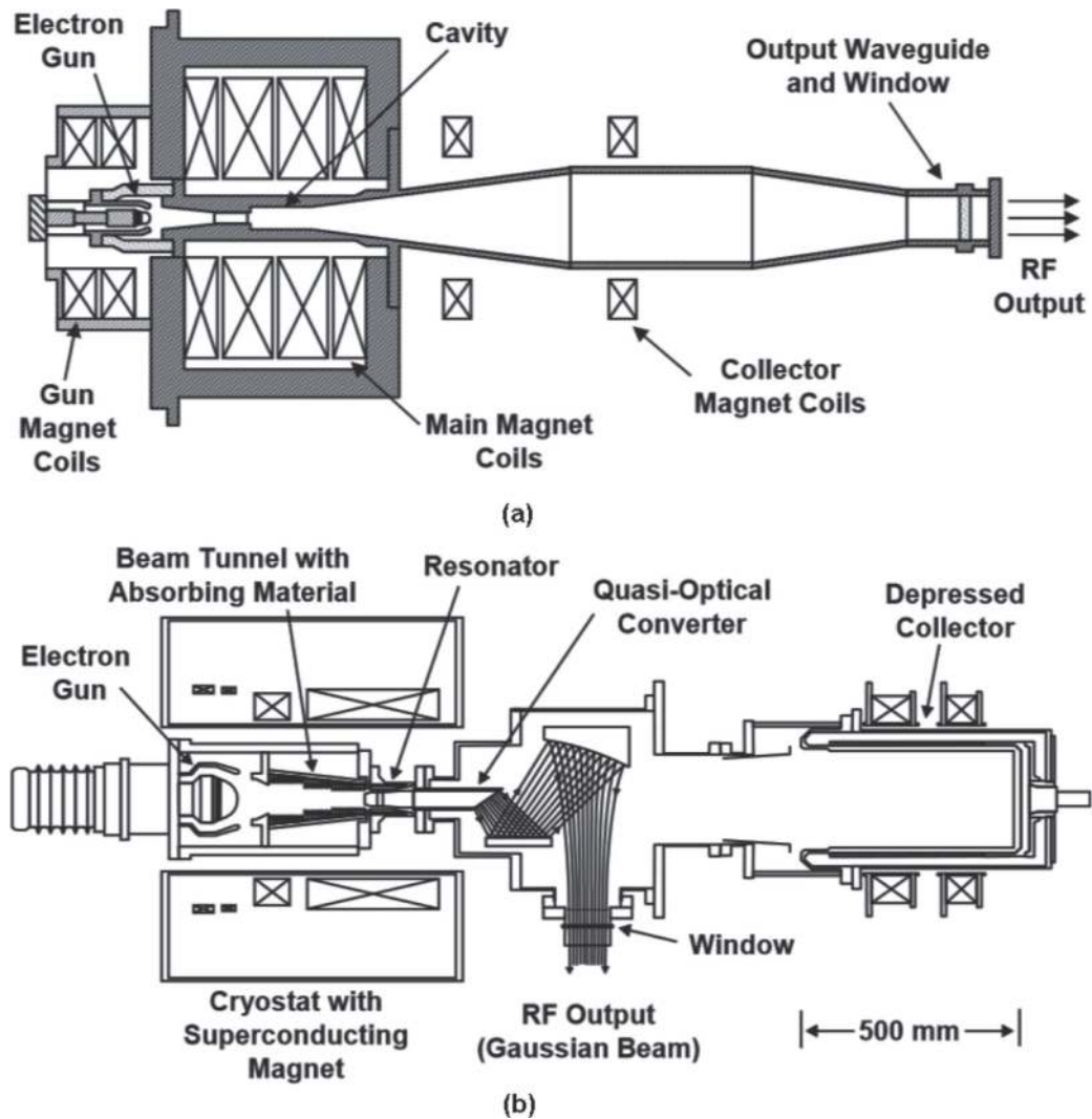
Figure 2. (a): Gyrotron with axial output. (b): High power Gyrotron with radial output of Gaussian beam.
