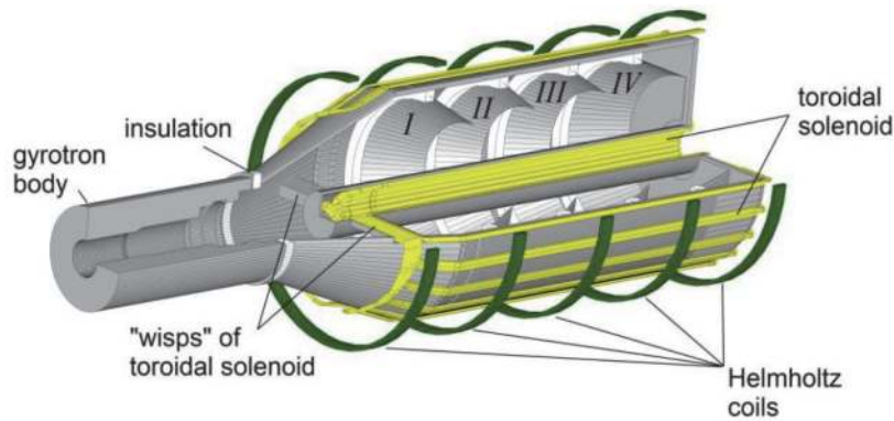
Figure 12. Cut-section view of a typical collector.
