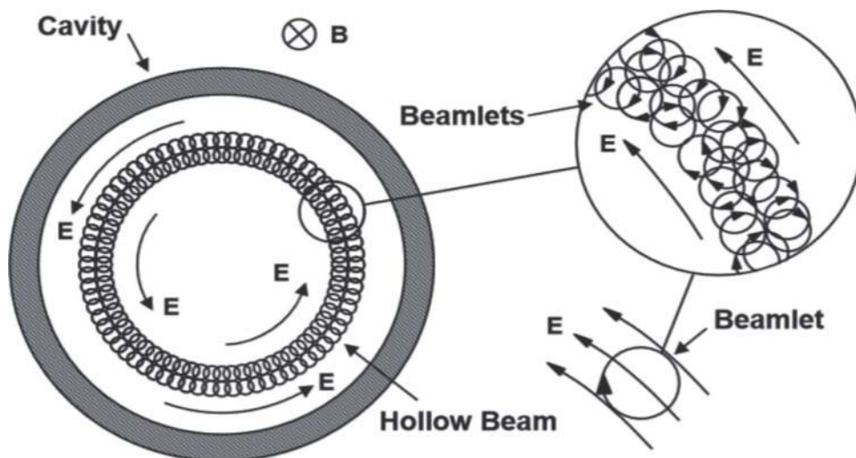
Figure 4. Gyrotron cross section showing electron trajectories.
