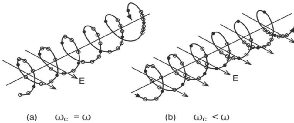
Figure 5. Bunching of electrons in a Gyrotron.
