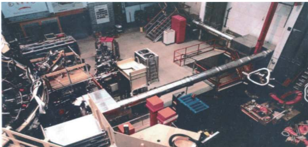
Figure 15. 140 GHz Gyrotron based ECRH system (Stellarator W7-AS).
