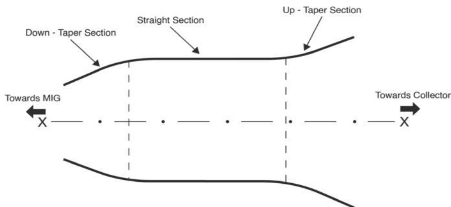
Figure 9. A typical Gyrotron cavity.
