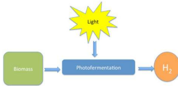
Figure 1. Photofermentative hydrogen production
