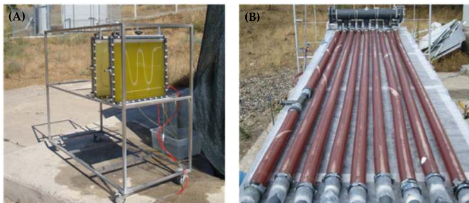
Figure 3. (A) Flat plate and (B) tubular photobioreactors.
