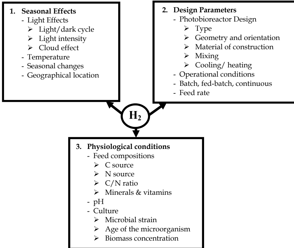
Figure 4. Parameters affecting photofermentative hydrogen production.
