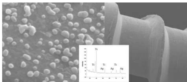
Figure 5. SEM images of silver nanoparticles deposited on the surface of the titanium screw, fixing the implant with the bone.
