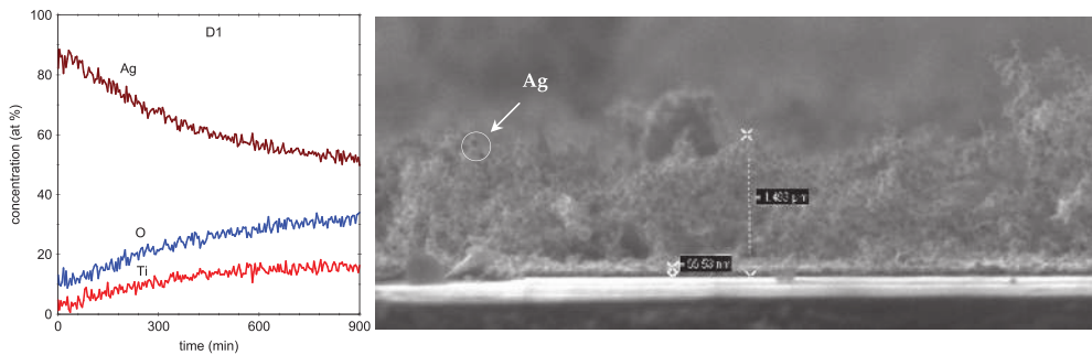
Figure 6. SEM images and XPS depth profile of the TiO 2 /Ag composite coating deposited on the surface of titanium implant (CVD, titania matrix were obtained using [Ti 6 O 9 (H 2 O) 2 (O t Bu) 6 (OOC t Bu) 6 ] as the precursor, T D = 713 K, p = 3 hPa, t = 60 min, Ar, and silver nanoparticles were deposited using [Ag(OOCC 2 H 5 t Bu)(PET 3 )] as the precursor, T D = 433 K, p = 1.5 hPa, t = 60 min, Ar) [52].
