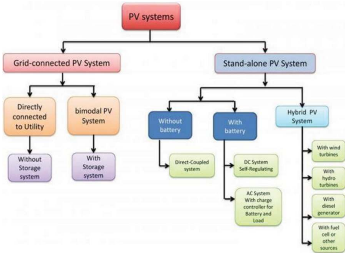
Figure 6. The different types of PV configurations [35].
