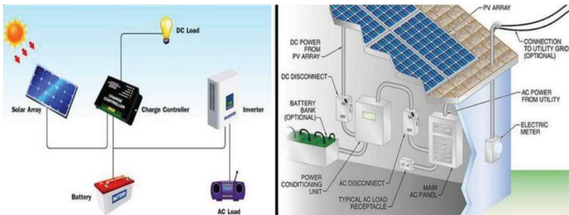
Figure 7. The photovoltaic solar system [38, 39].
