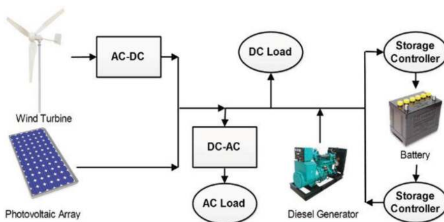
Figure 5. Hybrid renewable energy system (HRES) schematic [29].
