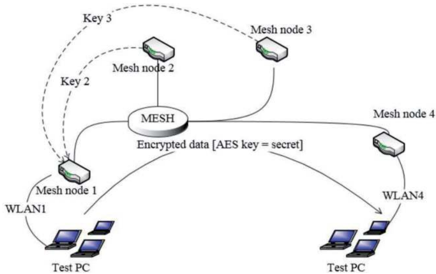
Figure 11. System model.
