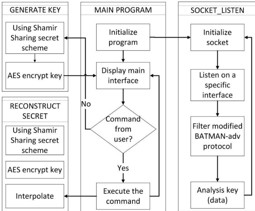
Figure 6. Proposed program flow graph.
