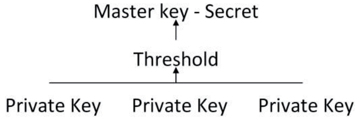
Figure 2. Proposed secret sharing scheme.
