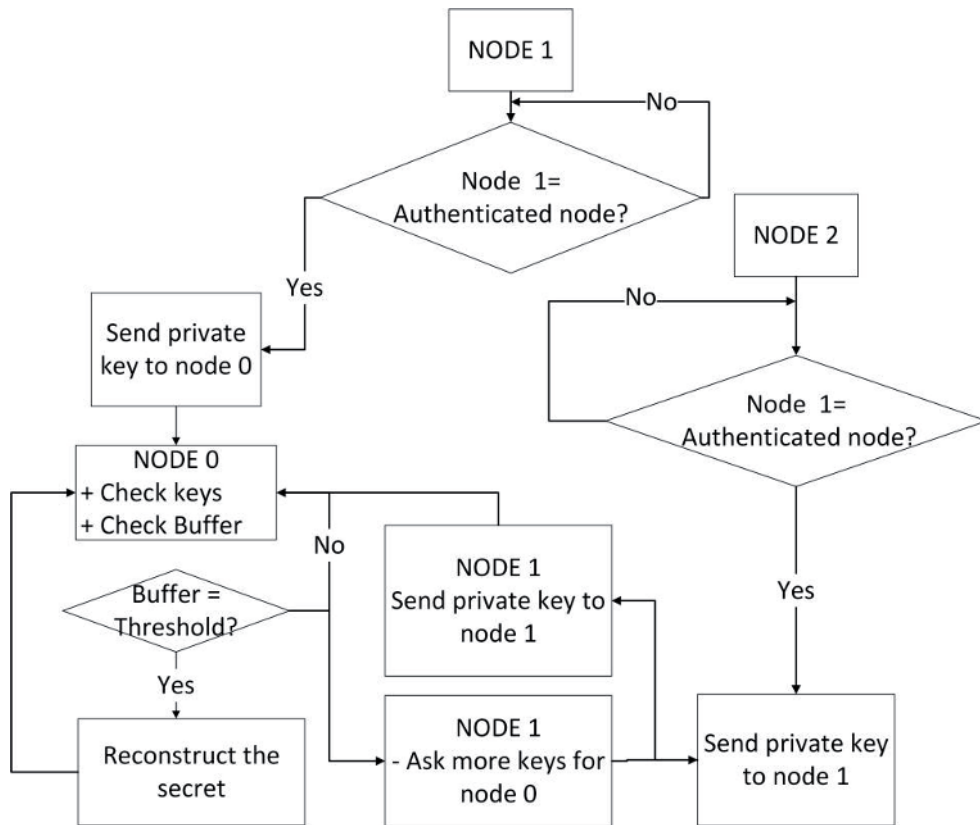
Figure 8. Secret reconstruction of node 0.
