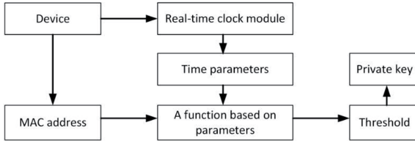
Figure 3. The process of private key generation.
