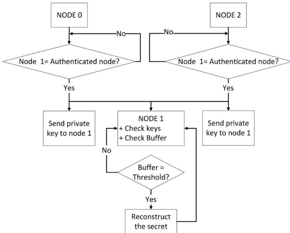
Figure 7. Secret reconstruction of node 1.
