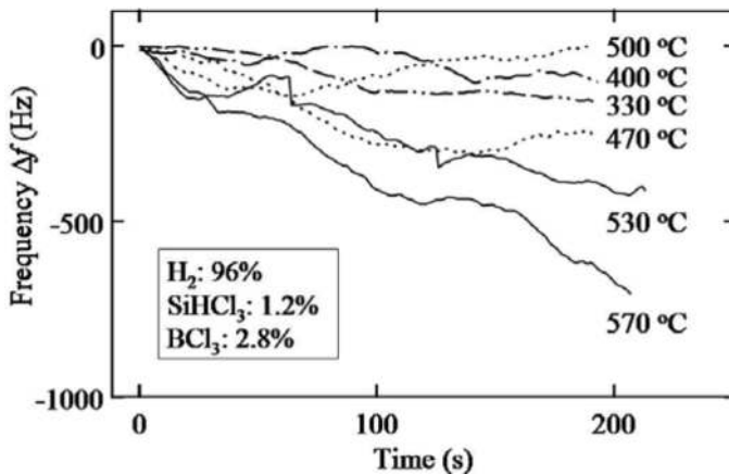
Figure 14. LCM frequency change at various trichlorosilane and boron trichloride concentrations at 330–570°C.
