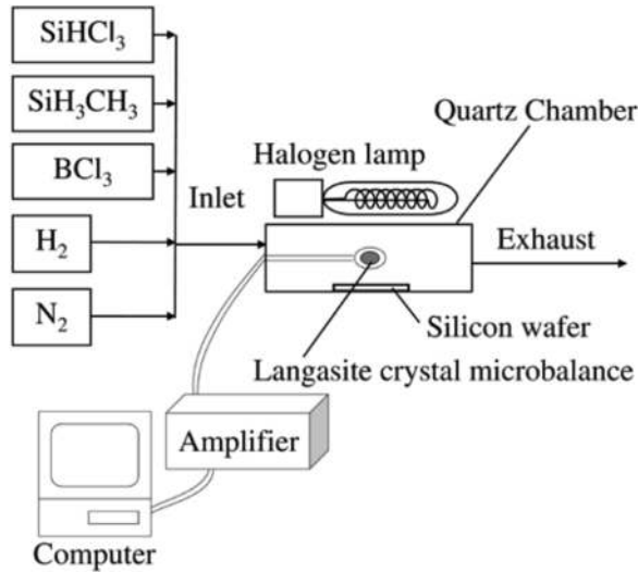
Figure 1. Chemical vapour deposition reactor containing a languasite crystal microbalance.
