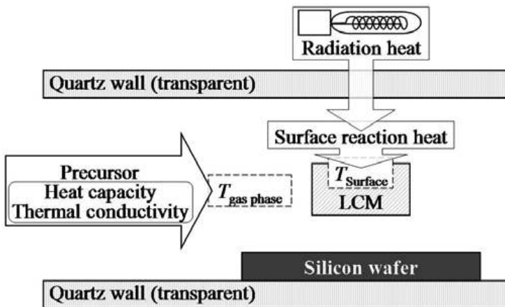
Figure 20. Parameters influencing the LCM temperature.
