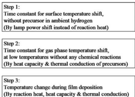
Figure 21. Three steps for evaluating temperature change during film deposition
