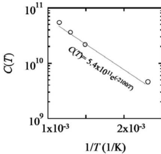
Figure 6. C(T) values changing with 1/T .
