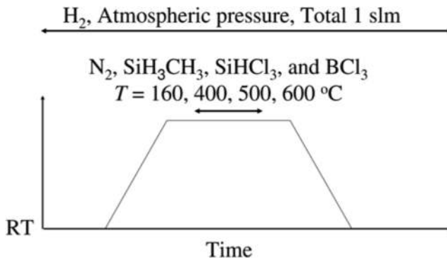
Figure 2. Process for measuring the frequency of the languasite crystal microbalance under various conditions.
