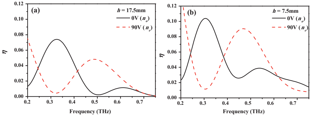
Figure 14. Diffraction efficiency of the devices with bases of (a) h = 17.5 mm and (b) h = 7.5 mm.
