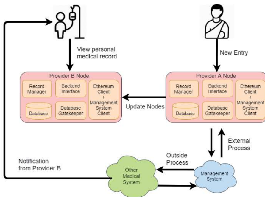
Figure 5. System workflow.
