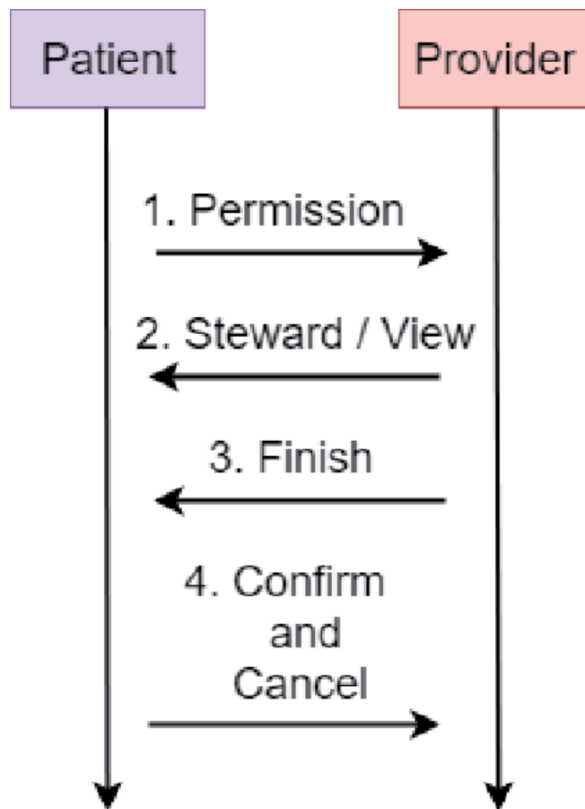
Figure 2. Authorization procedure of getting medical record permission.
