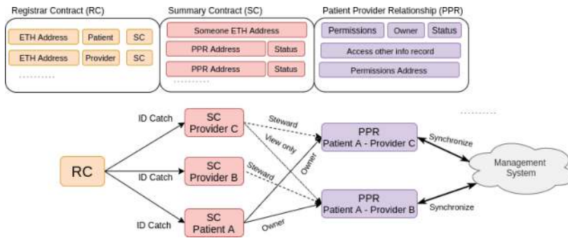
Figure 1. Proposed smart contract-based medical management system.
