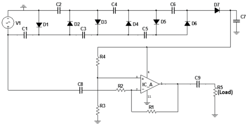
Figure 13. AC voltage booster circuit.
