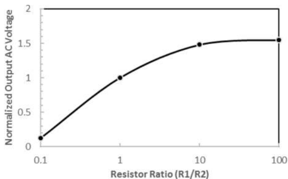
Figure 16. Measured output AC voltage with normalization.
