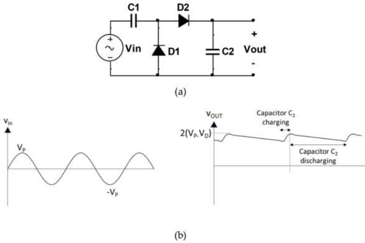
Figure 2. (a) Greinacher voltage doubler circuit and (b) it's corresponding input/output waveform.
