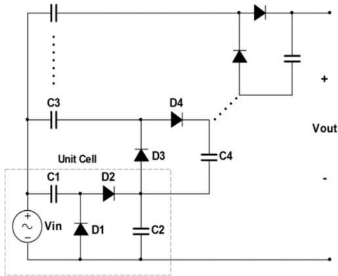
Figure 9. Modified Karthaus-Fischer cascade voltage multiplier circuit.
