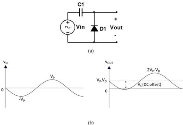
Figure 1. (a) Villard voltage doubler circuit and (b) its corresponding input/output waveform [8].
