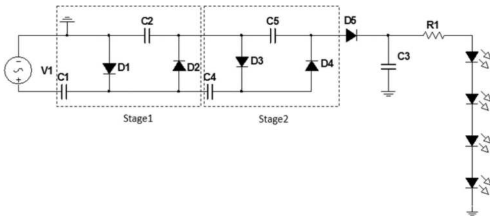
Figure 11. Quadriplier voltage generator circuit.
