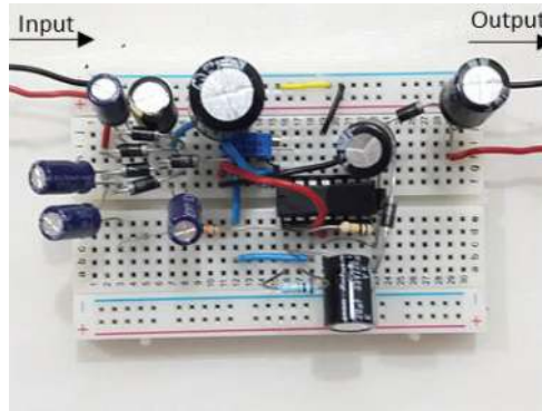
Figure 19. Circuit photo of variable voltage generator.
