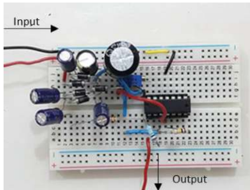
Figure 15. Circuit photo of AC voltage booster.
