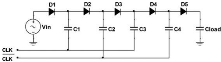
Figure 6. Dickson charge pump circuit.
