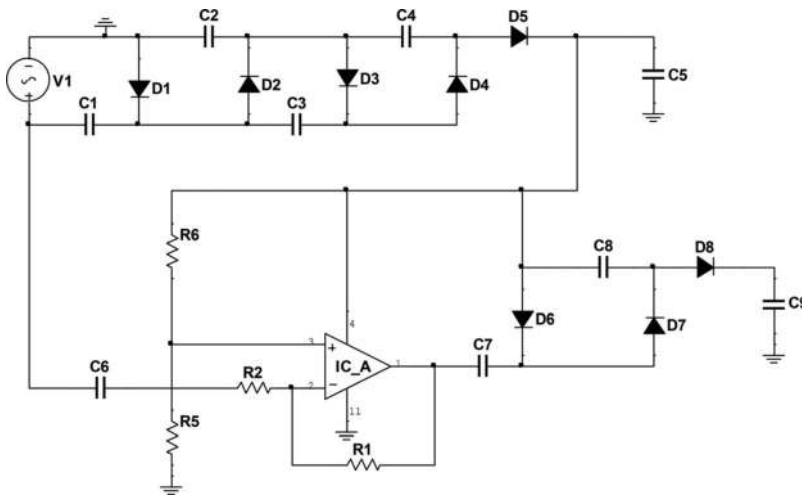
Figure 17. Variable DC voltage generator.
