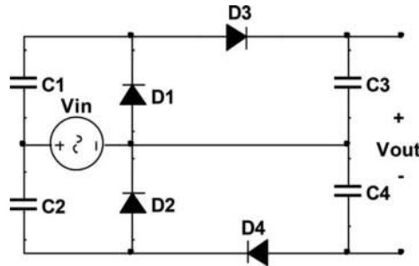
Figure 5. Full-wave Greinacher voltage doubler circuit.
