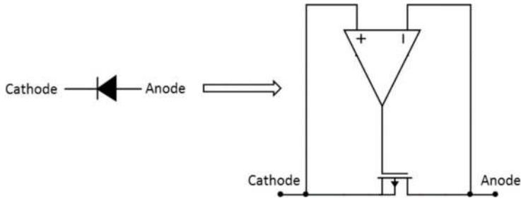
Figure 10. Active diode circuit.
