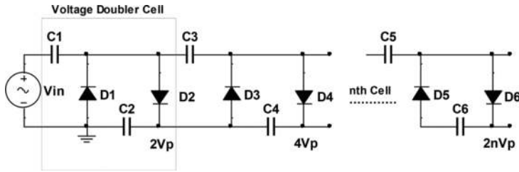
Figure 3. N-stage Cockcroft-Walton voltage multiplier circuit [10].
