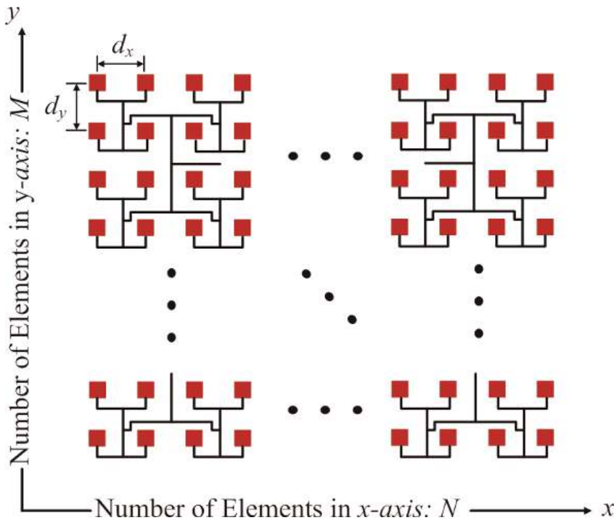
Figure 13. Layout of the feed network.
