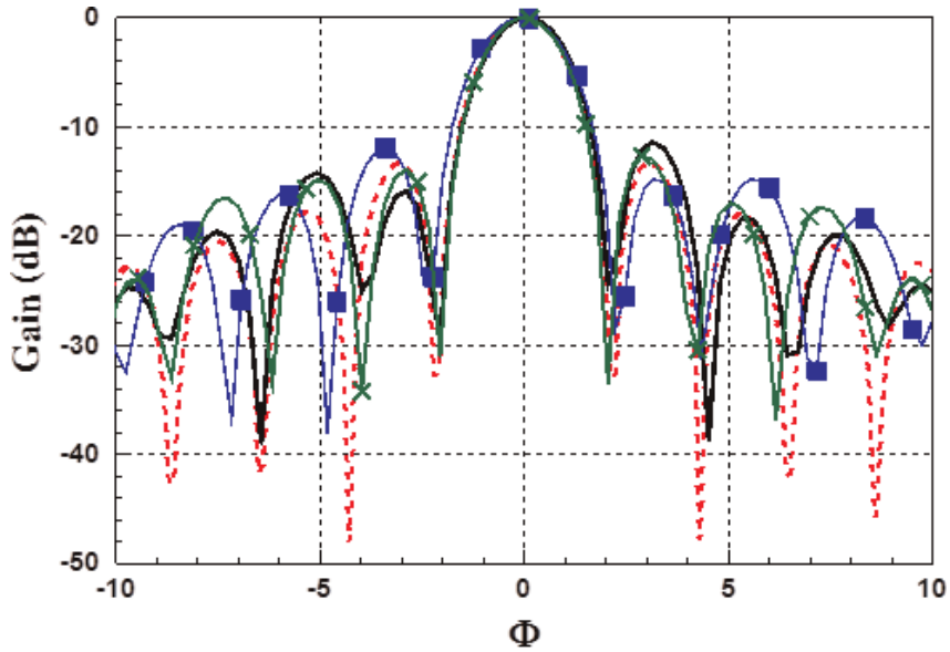
Figure 25. Radiation pattern of vertical polarized full array in azimuth plane ( \theta = 20^\circ cut). ( — Measured @ 11.9 GHz, - - Simulated @ 11.9 GHz, —■— Measured @ 10.8 GHz, —×— Measured @ 12.8 GHz).
