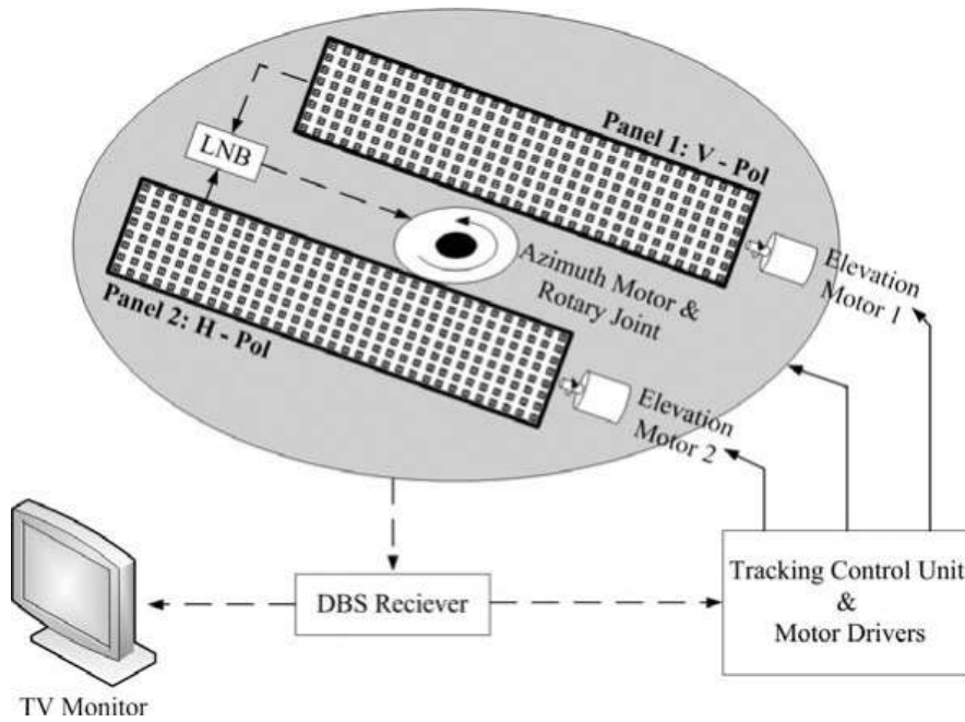
Figure 1. System configuration of the proposed array antenna.
