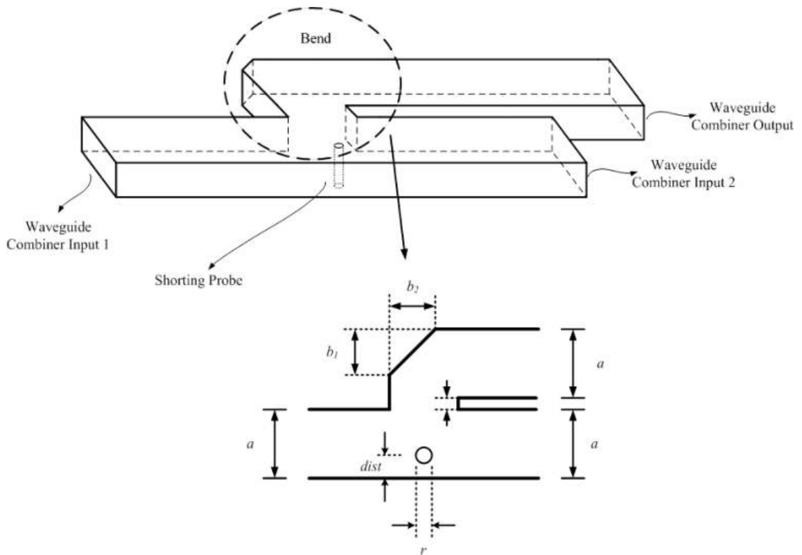
Figure 19. Waveguide bends and junctions.
