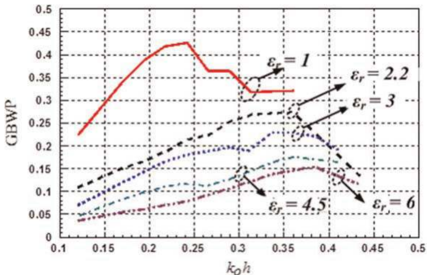
Figure 2. GBWP vs. k_0h . for different dielectric materials.
