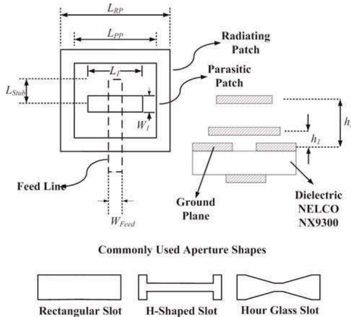
Figure 5. Aperture-coupled antenna and possible aperture shapes.
