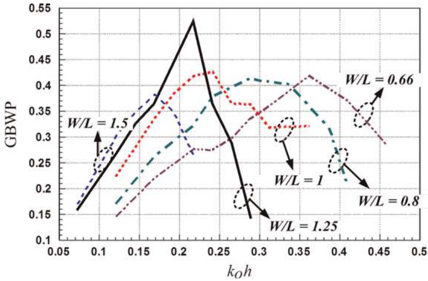
Figure 3. GBWP vs. k_0h for different aspect ratios.
