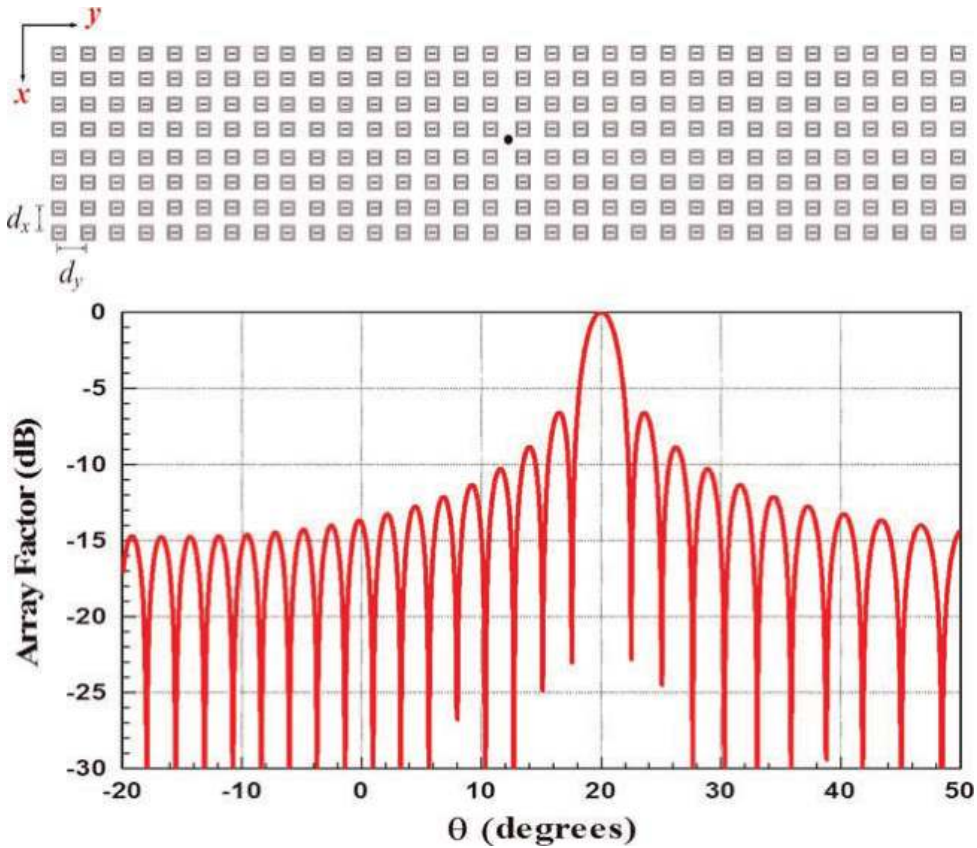
Figure 11. Array factor elevation pattern of synthesized array.
