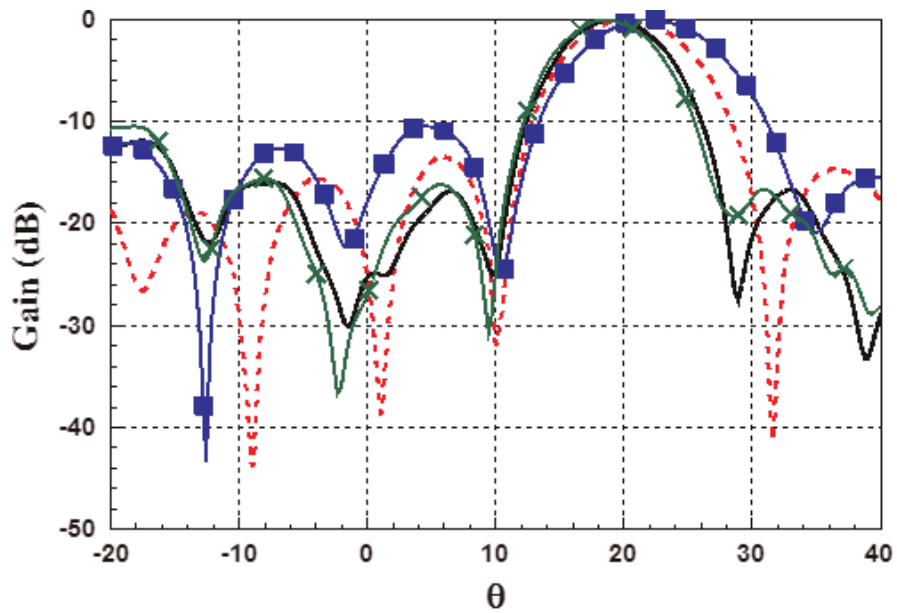
Figure 26. Radiation pattern of vertically polarized full array in \varphi -plane ( \varphi=0^\circ cut) ( — Measured @ 11.9 GHz, - - Simulated @ 11.9 GHz, ■ Measured @ 10.8 GHz, × Measured @ 12.8 GHz).
