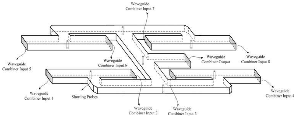
Figure 18. 8-to-1 power combiner.
