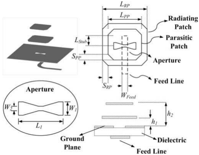
Figure 6. Aperture-coupled stacked microstrip patch antenna.
