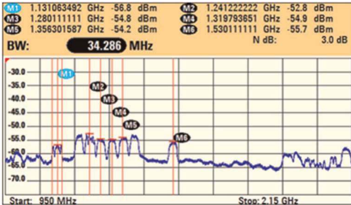
Figure 28. Spectrum analyser measurement of DBS signal.
