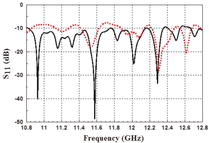
Figure 23. S11 of array antenna. (— Measured, - - - Simulated).
