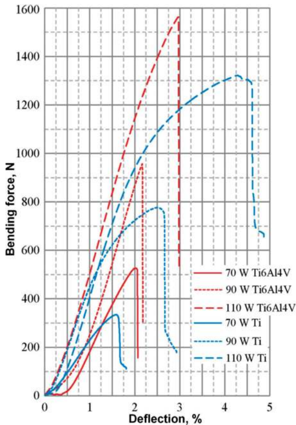
Figure 10. Comparison of diagrams of dependency between bending strength and bending of solid bridge no. 2 manufactured by SLS from titanium and Ti6Al4V alloy for different laser power.
