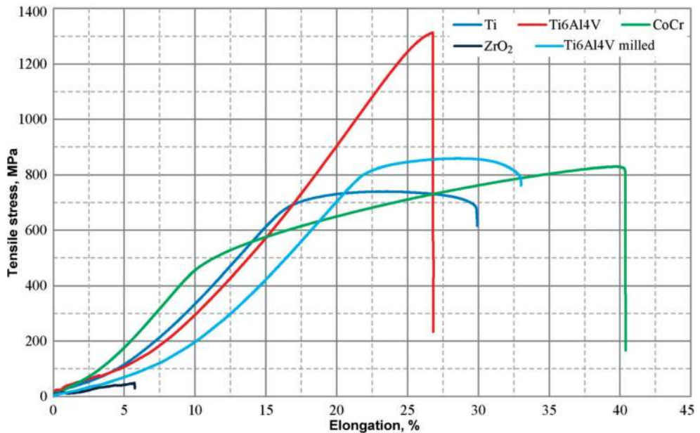
Figure 5. Comparison of diagrams of dependency between tensile stress and elongation for various examined materials, that is, for sintered Ti, sintered Ti6Al4V alloy, milled Co-Cr alloy, milled ZrO 2 sinter and milled Ti6Al4V alloy.
