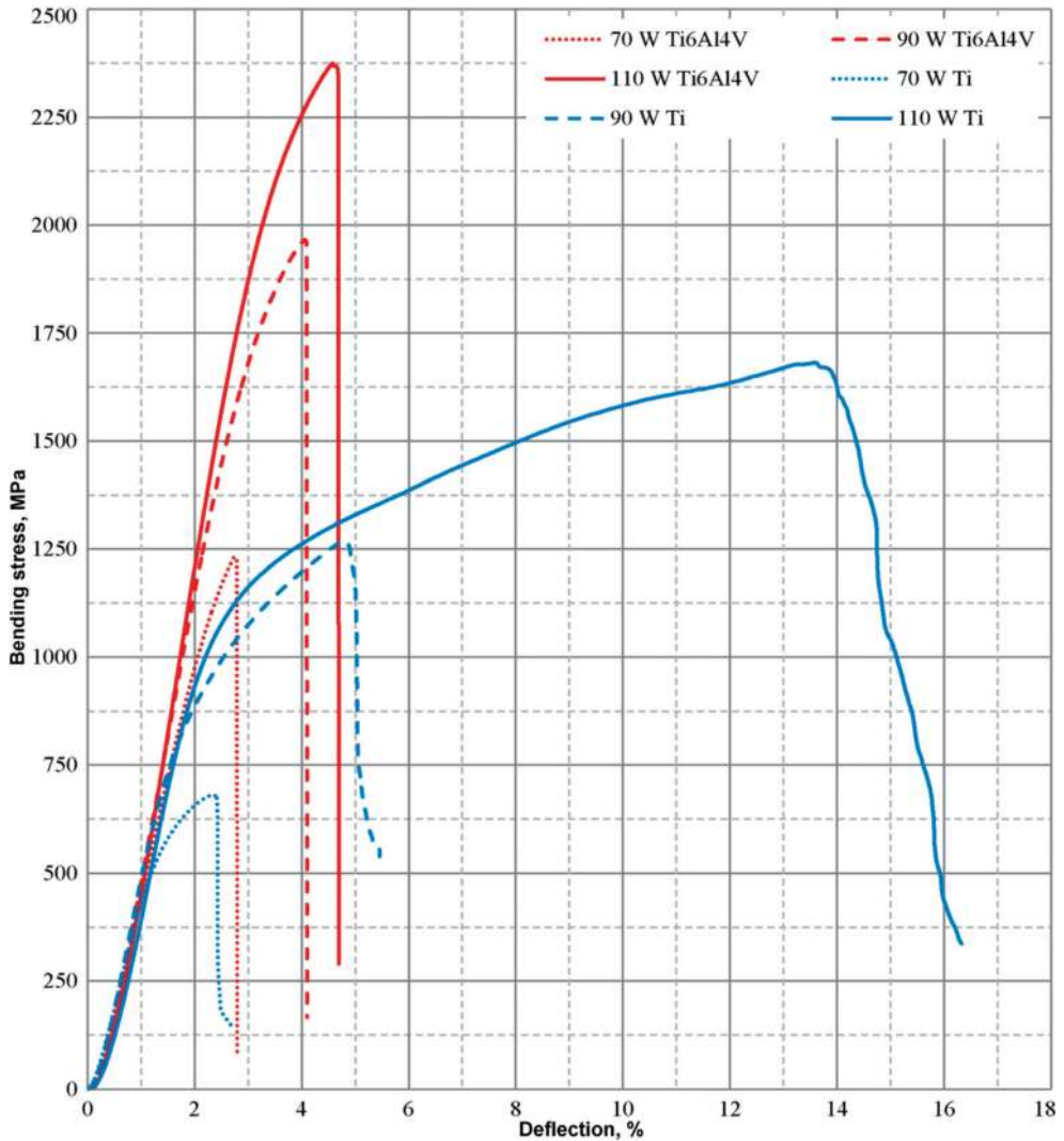
Figure 6. Comparison of diagrams of dependency between bending stress and bending for solid samples made of Ti6Al4V alloy and pristine titanium sintered at different laser powers.
