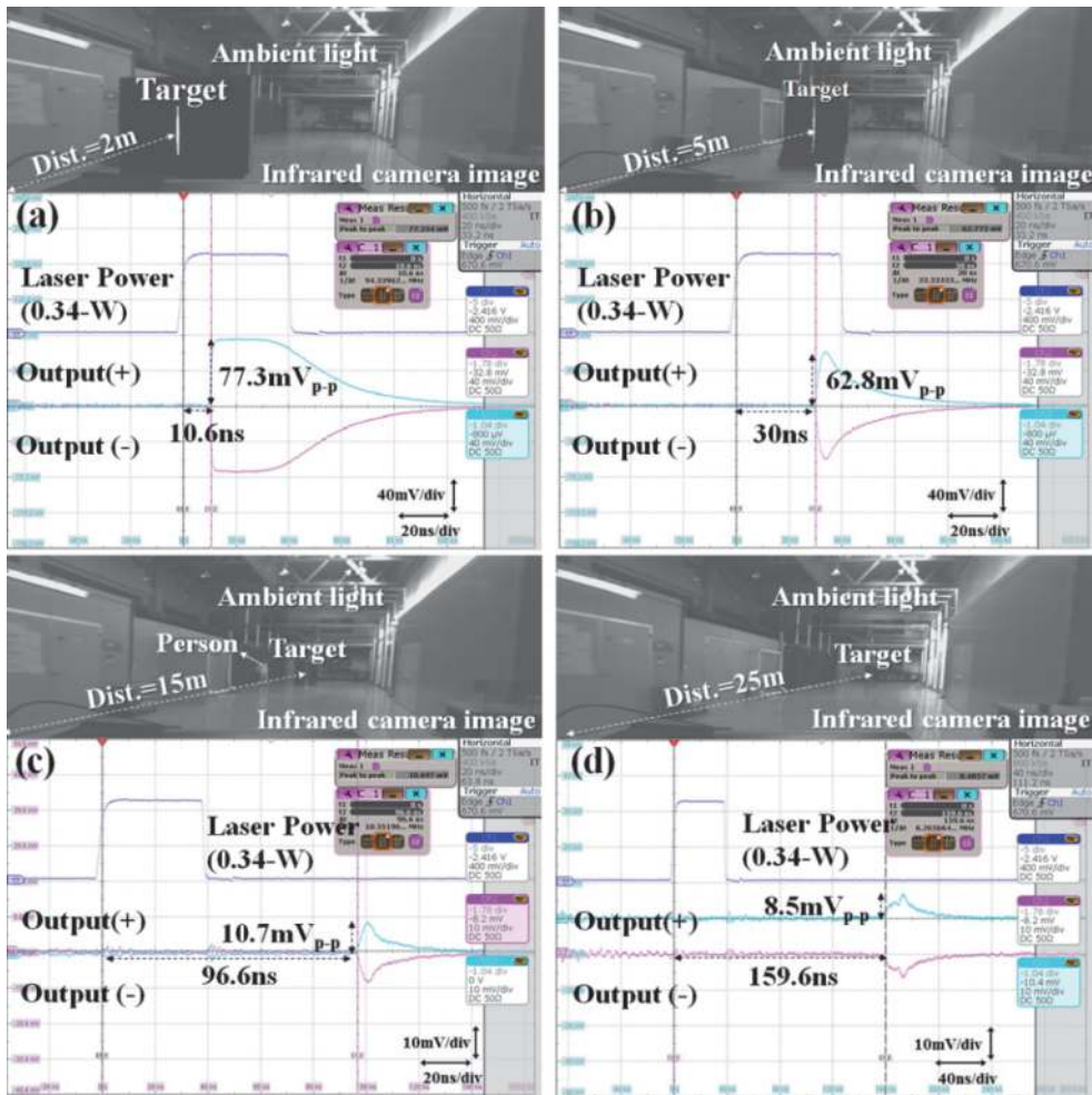
Figure 11. Recovered output pulses from 2 to 25 m.
