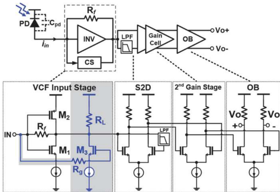
Figure 9. Schematic diagram of the VCF-TIA.
