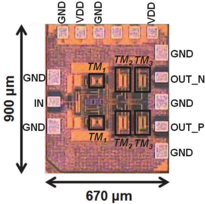
Figure 16. Chip microphotograph of the MC-TIA.
