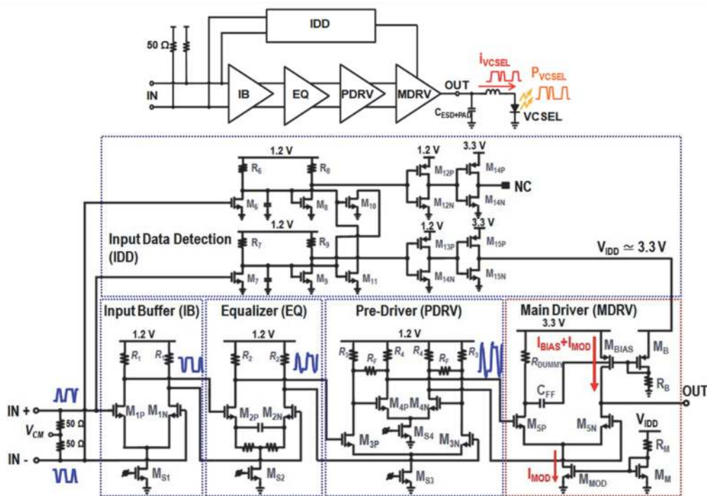
Figure 2. Schematic diagram of the VCSEL driver.
