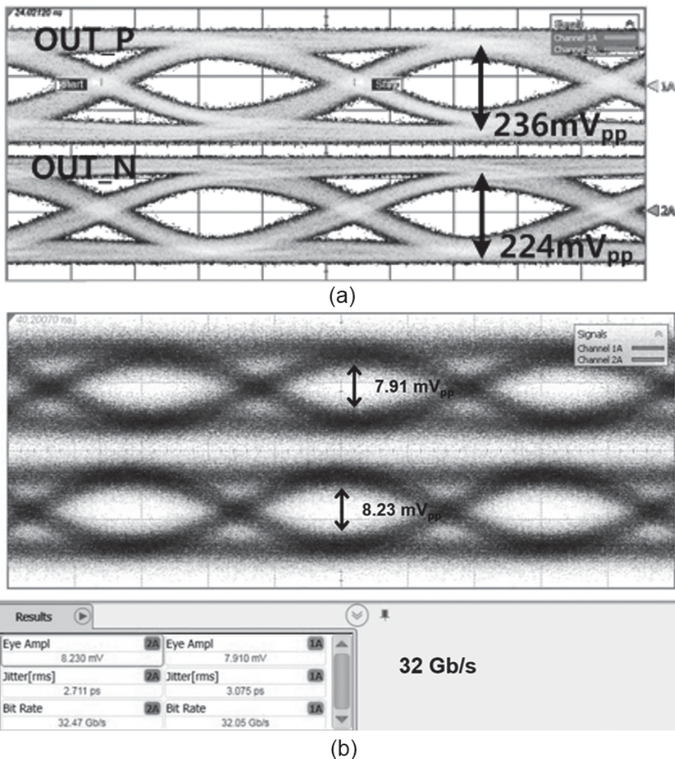
Figure 18. Measured eye diagrams of the MC-TIA (a) with 1.5 \text{ mA}_{pp} and (b) 100 \text{ }\mu\text{A}_{pp} input currents, respectively.
