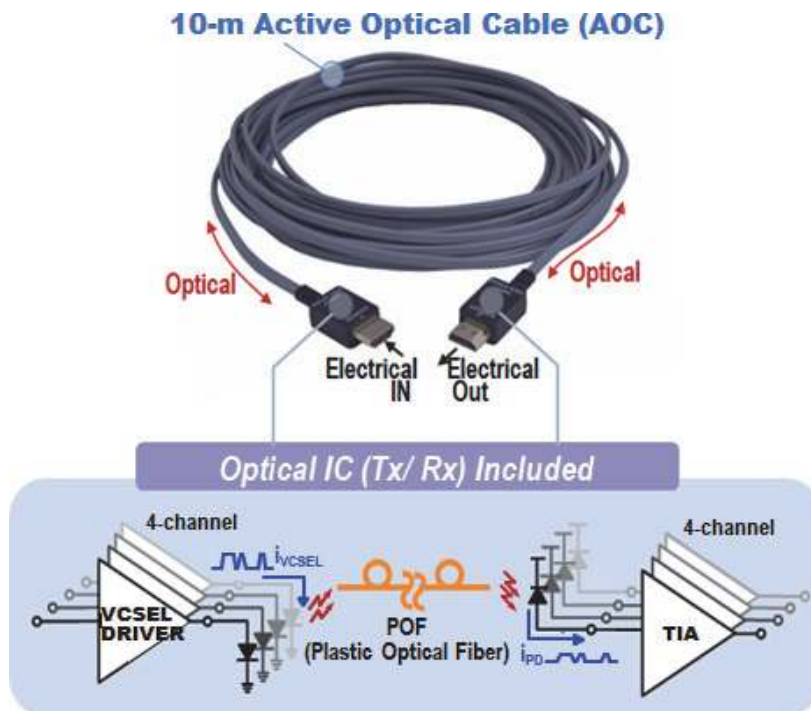
Figure 1. Block diagram of the 4-channel optical ICs.
