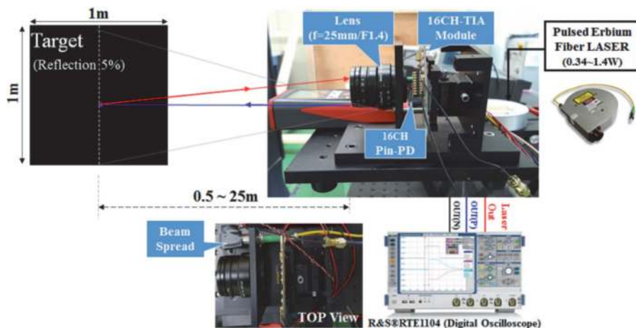
Figure 10. Test setup of the 16-channel VCF-TIA array.
