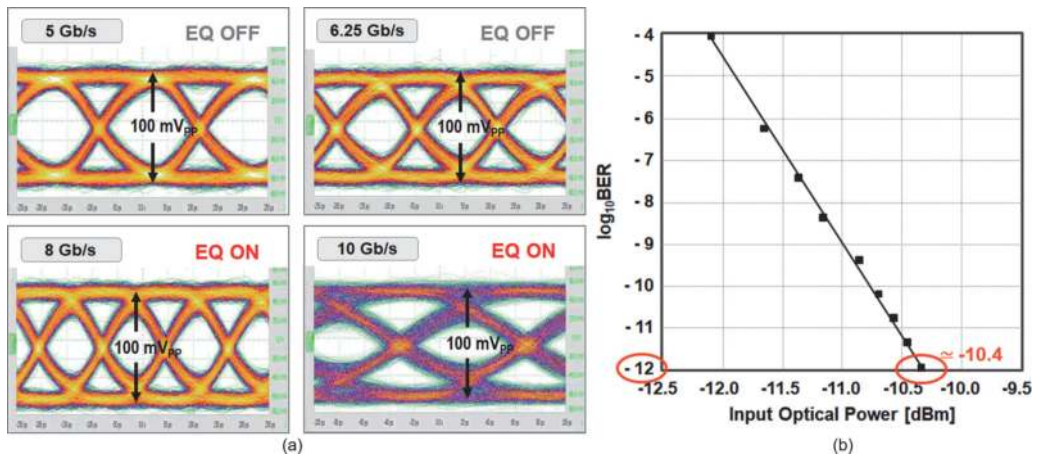
Figure 7. Measured eye diagrams.
