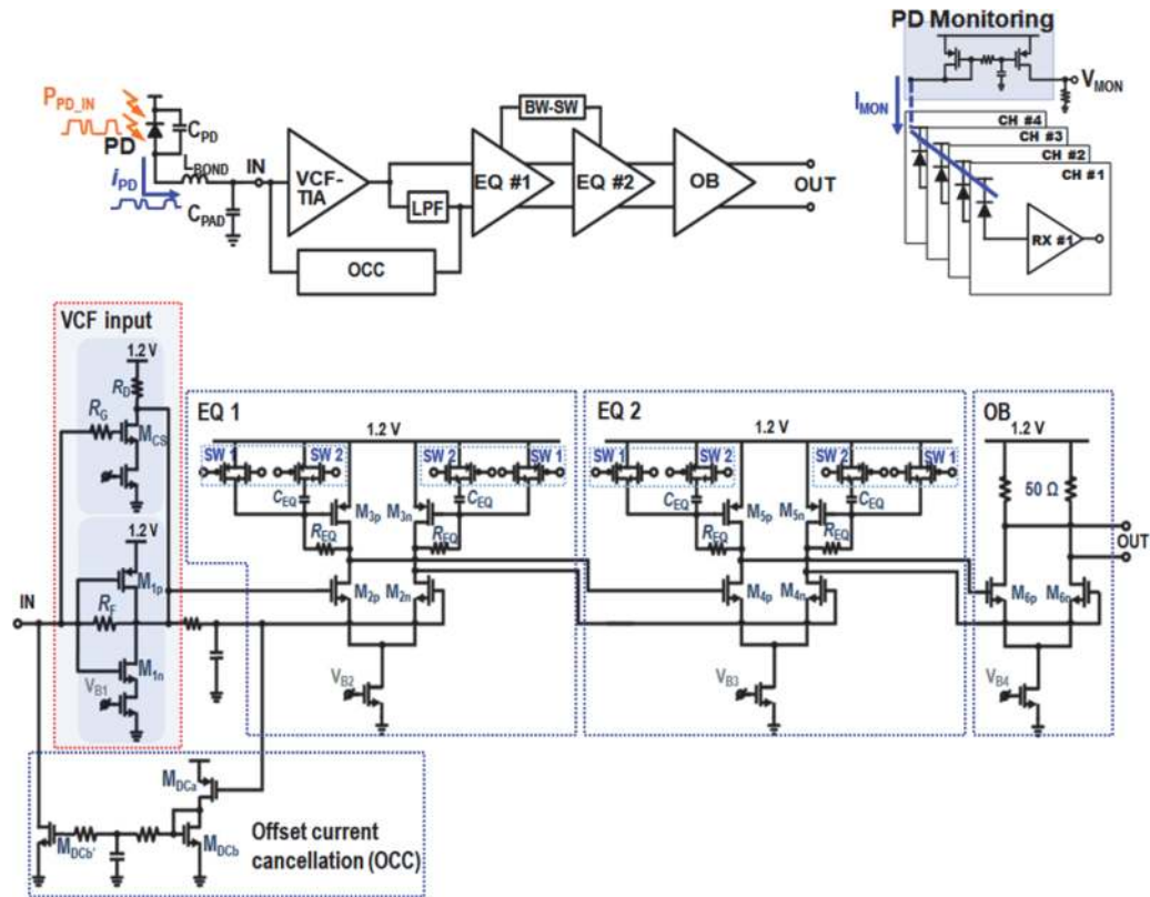
Figure 5. Schematic diagram of the VCF-TIA.
