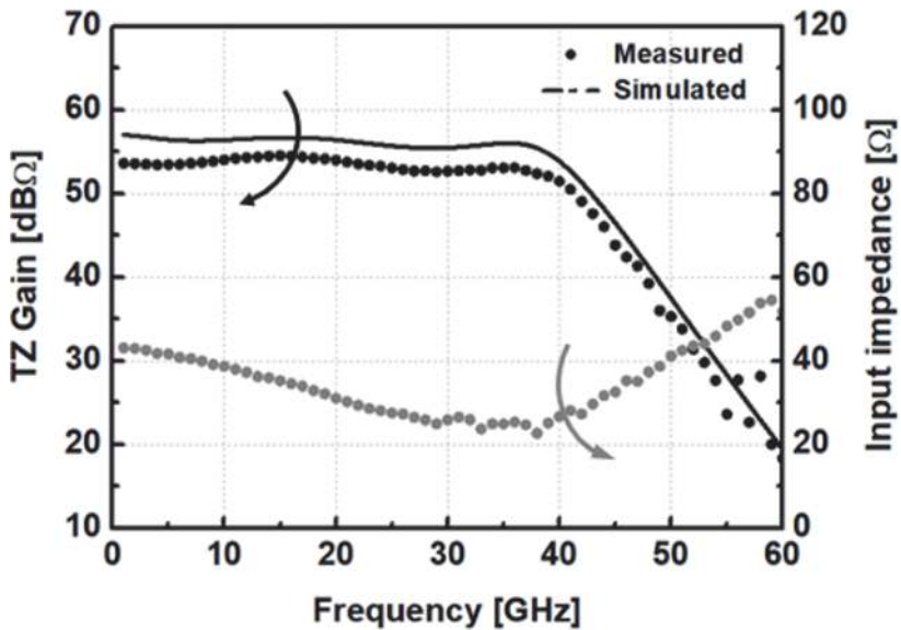
Figure 17. Measured frequency response of the MC-TIA.
