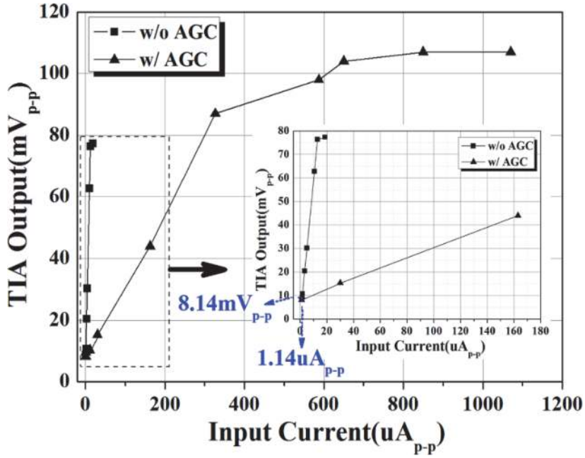
Figure 13. Measured transimpedance gain with AGC.
