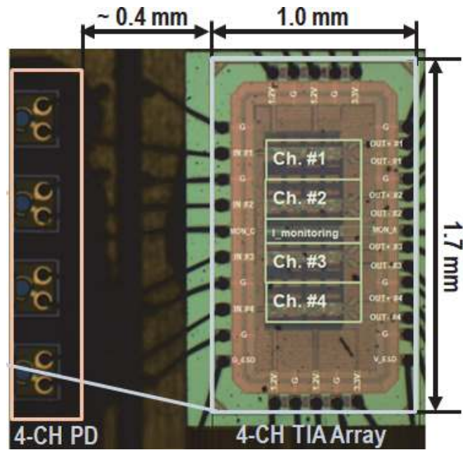
Figure 6. Chip microphotograph of the 4-channel VCF-TIA array.
