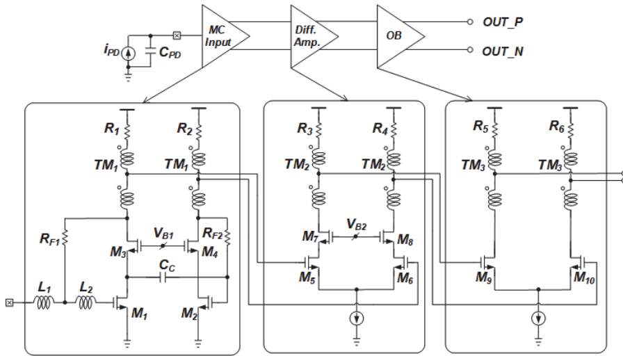
Figure 14. Schematic diagram of the MC-TIA.
