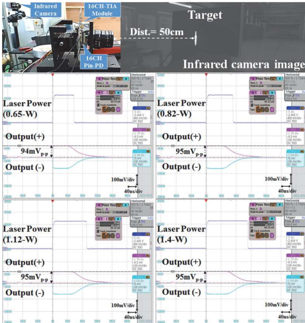
Figure 12. Recovered output pulses within 0.5 m.
