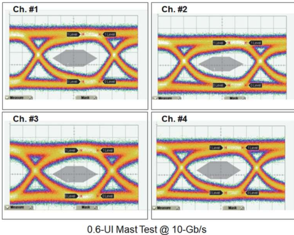
Figure 4. 4-channel eye mask at 10 Gb/s.
