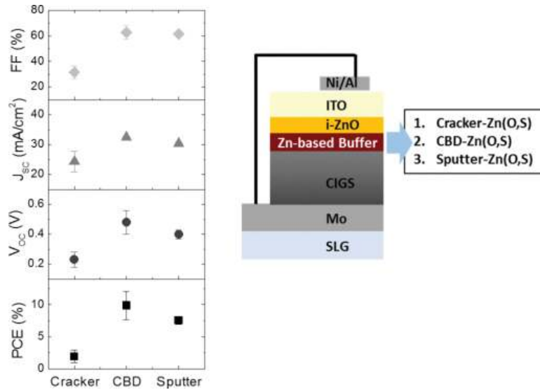
Figure 8. The performance of the CIGS solar cell as a function of the method of deposition of the Zn-based buffer layer (left), and an illustration of the completed CIGS solar cell structure (right).
