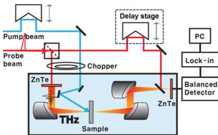
Figure 2. Schematic diagram of OPTP measurement system.
