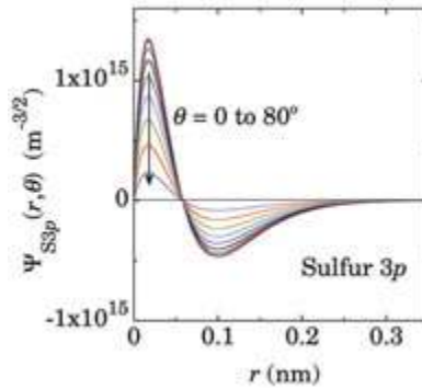
Figure 3. 3p wavefunction of a sulfur atom with the effective nuclear charge of Z_{eff} = 5.48 for every 10^\circ of \theta from 0 to 80, which is defined in Figure 4 . r is the distance from the sulfur nucleus. STM usually observes the region much farther than 0.1 nm (reused from Ref. [1]).
