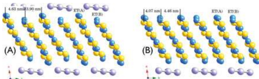
Figure 13. (A) Crystal structure of \beta\text{-(ET)}_2\text{I}_3 projected along the c axis with three unit cells. ET(A) is located nearer to the b - c surface by \approx 0.1 nm than ET(B). (B) A model for the surface layer of \beta\text{-(ET)}_2\text{I}_3 . ET(B)s are slid to align TTF double bonds to the same height as that of ET(A), which increases the cohesive energy in the surface ET layer. The separations between ET(A) and ET(B) are contrasted to (A). The topmost sulfur atoms of ET(B) are slightly deeper by 0.01 nm than ET(A).
