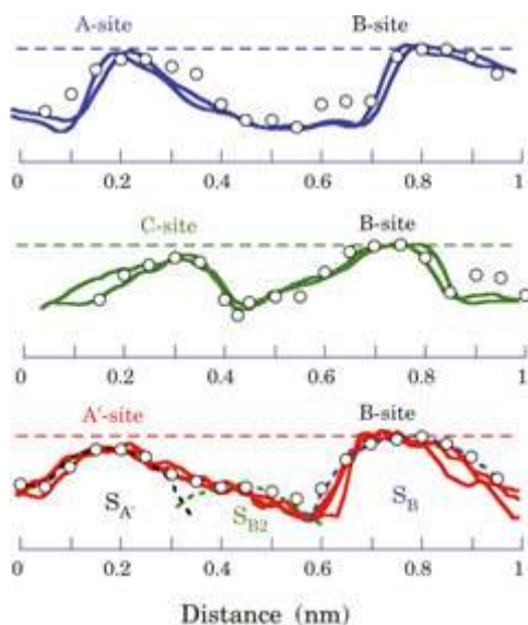
Figure 10. STM topographies of \alpha -(BEDT-TTF) 2 I 3 (solid curves) and the simulations (open circles) with \sum_i |\Psi_{S3p}^i|^2 , where the molecular charge ratio \rho_i / \rho_B in Table 1 was taken into account. The topographies were measured along the arrows in Figure 9(B) . The horizontal dashed straight lines are visual guides at the top of the S_B site. The broken curves for the bottom A–B scan show individual contributions of each sulfur atom at S_B and S_{A'} and S_{B2} . From S_{B'} , note that S_{B2} is 0.1 nm inside. The vertical scale is the same as the horizontal one (reused from Ref. [1]).
