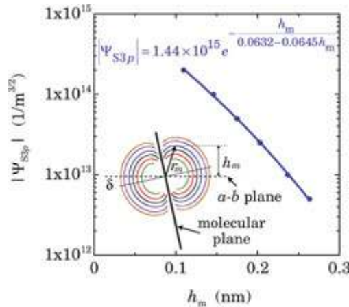
Figure 5. Maximum height h_m estimated from each \Psi_{S3p} wavefunction contour in the inset, where the symmetry axis (thin solid line) of the 3 p wavefunction tilts by \delta \approx 12 deg against the a - b plane described by the dashed horizontal line through the sulfur atom. The analytical expression approximately describes |\Psi_{S3p}| as a function of h_m , which is applicable to the STM topography analysis in the a - b plane of \alpha -(ET) 2 I 3 (reused from Ref. [1]).
