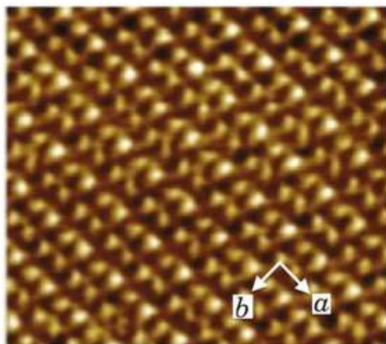
Figure 8. STM image of a thin plate-like single crystal of \alpha -(BEDT-TTF) 2 I 3 in \approx 7.0 \times 6.5 \text{ nm}^2 , where the thermal drift was corrected with the reported lattice parameters [23]. The assigned a and b axes are indicated by the arrows (reused from Ref. [1]).
