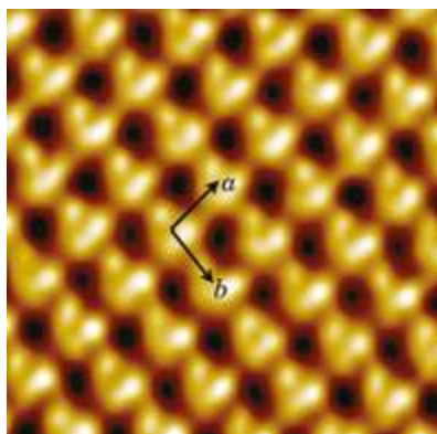
Figure 18. STM image of a single crystal of (EDO-TTF) 2 PF 6 in 4.7 × 4.7 nm 2 with the setpoint of 6.1 pA and the tip potential of 200 mV. Thermal drift was corrected with reference to the reported crystal structure [21] and FFT filter was applied. The assigned a and b axes are shown by the arrows.
