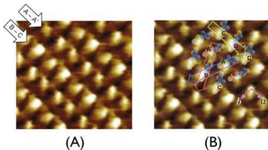
Figure 9. STM image of \alpha -(BEDT-TTF) _2 I _3 in 2.8 \times 2.6 .nm ^2 . Four BEDT-TTF molecules are contained in the unit cell. (A) Molecular arrays, A-A' and B-C, run from the top left to the right bottom. (B) Crystal structure assigned to the STM image of \alpha -(BEDT-TTF) _2 I _3 . The balls with A', A, B, and C represent the relevant sulfur atoms. The three large arrows represent the direction of the topography shown in Figure 10 (reused from Ref. [1]).
