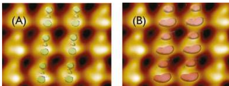
Figure 19. STM image of (EDO-TTF) 2 PF 6 with (A) the simulated constant charge density contour of 3 \times 10^{-8} \text{ nm}^{-3} at 2 Å from the oxygen atom. The second oxygen and the second carbon contribute only a little. The small spots are assigned to the second half of O 2p orbital and with (B) the simulation by the rotational reconstruction model with the condition of \theta_a = 18^\circ , \theta_b = 29^\circ as described in Figure 20, which successfully reproduces the overall profile of the observed image.
