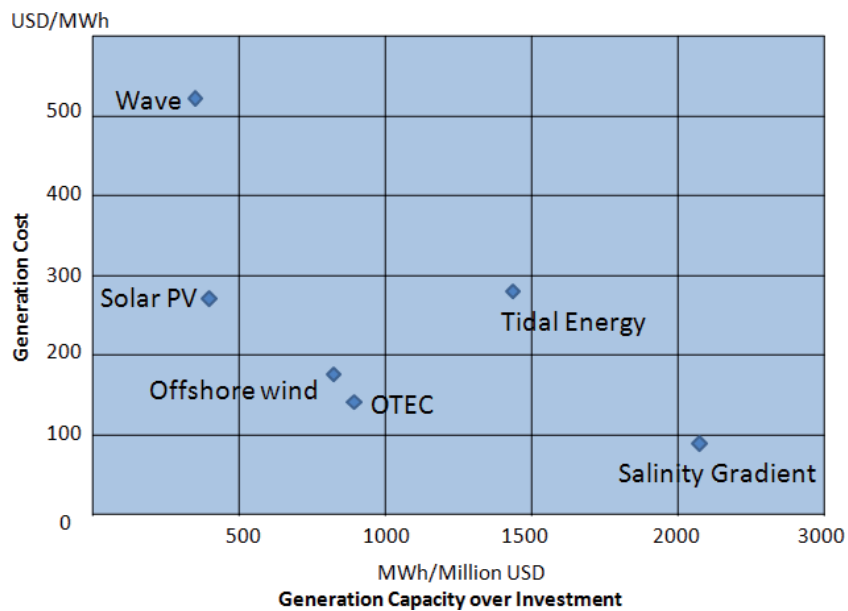
Figure 6. Comparative analysis of various forms of renewable energy (RE) [14].
