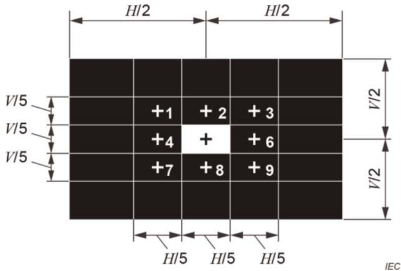
Figure 16. Test pattern for local contrast.
