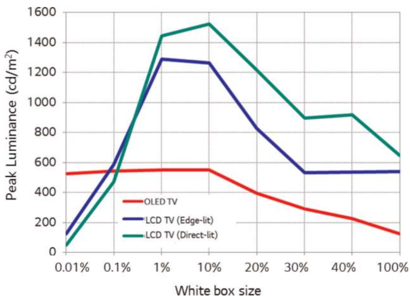
Figure 13. Peak luminance of the OLED TV and the LCD TVs according to the size of the white boxes.
