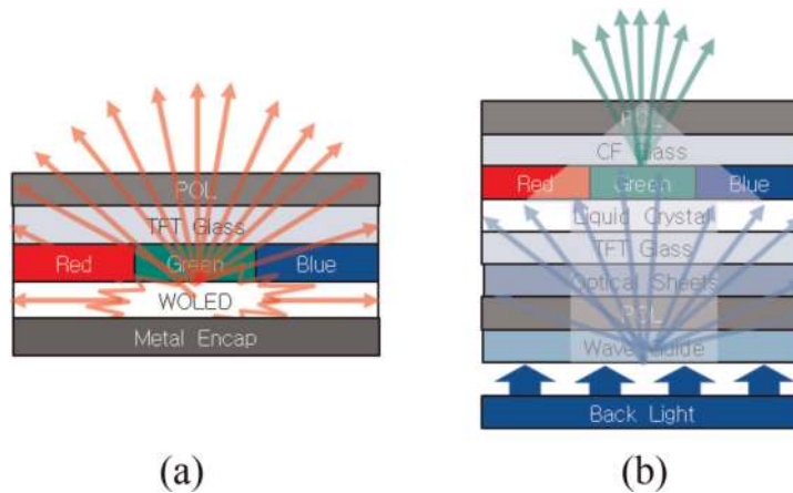
Figure 17. Conceptual diagrams of light path of OLED TV and LCD TV. (a) OLED TV and (b) LCD TV.
