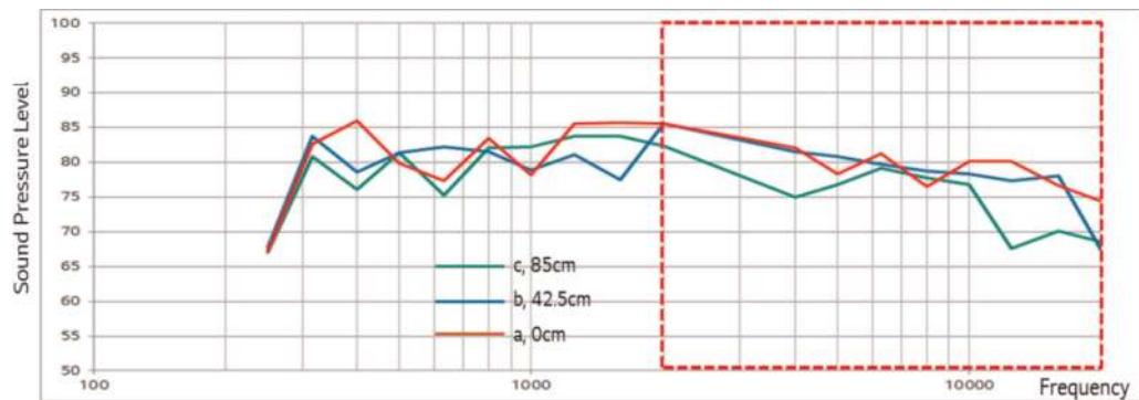
Figure 20. Frequency response results by speaker height.
