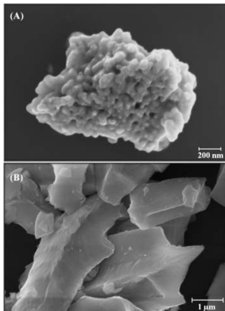
Figure 7. HR-SEM micrograph of BCT20 powders heat treated at (A) 500 °C and (B) 600 °C for 2 h.
