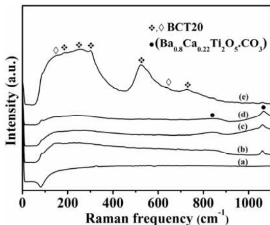
Figure 6. Spontaneous Raman spectra of BCT20 powders heat treated at (a) 400°C, (b) 500°C, (c) 550°C, (d) 575°C and (e) 600°C
