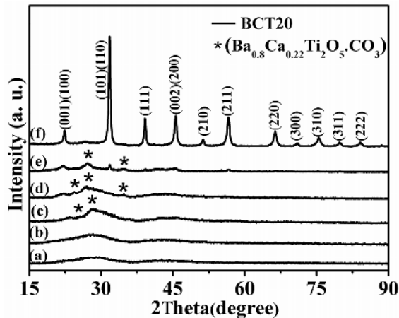
Figure 5. XRD patterns of the BCT powders calcined at temperatures: (a) 400°C; (b) 450°C; (c) 500°C; (d) 550°C; (e) 575°C and (f) 600°C.
