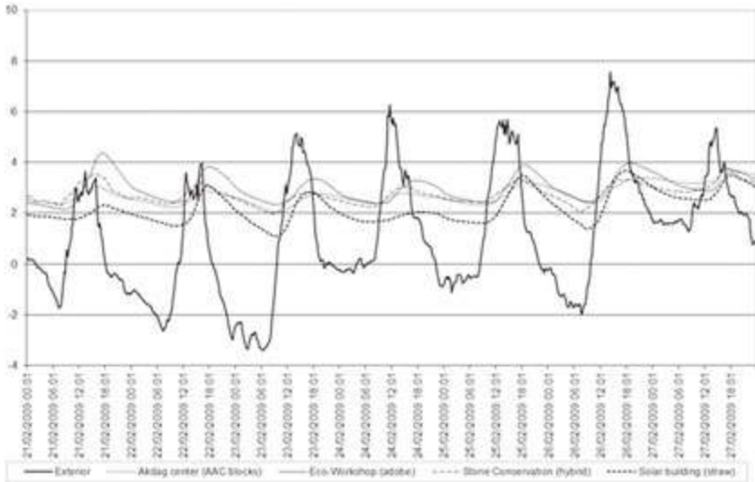
Figure 13. Comparison of thermal performance of the buildings in Kerkenes Eco-Center.
