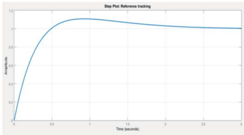
Figure 5. PID step response optimization.
