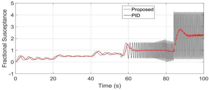
Figure 12. Control signal comparison.
