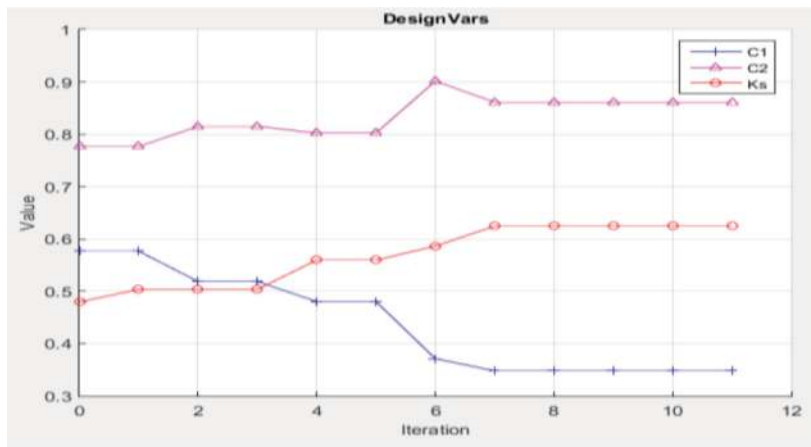
Figure 3. Optimized parameters of the proposed scheme.
