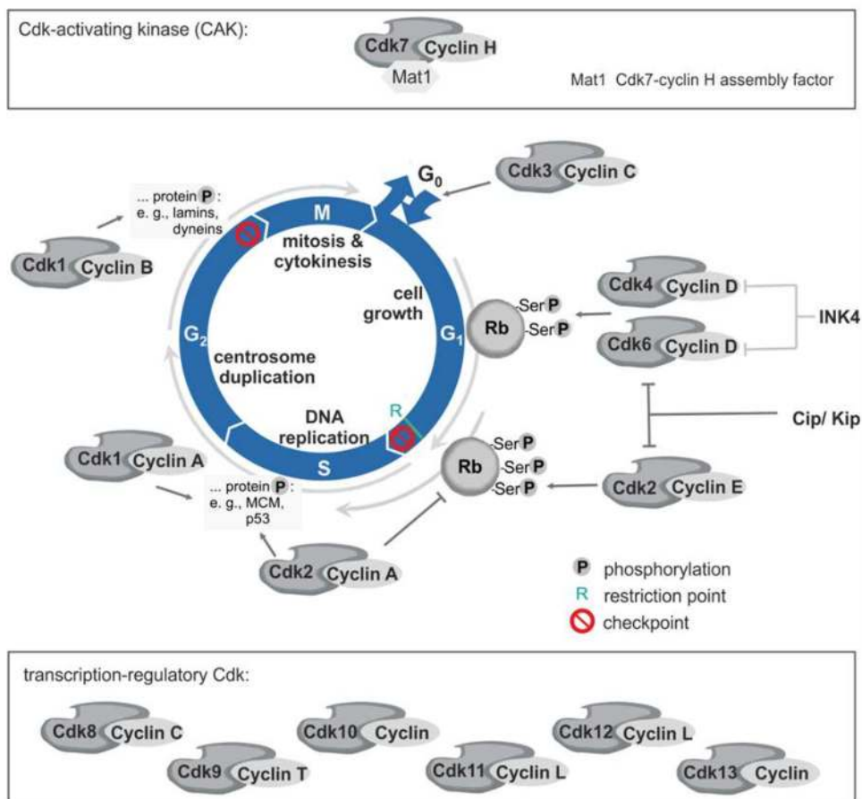
Fig. 1. Overview of human cell cycle activation and transcriptional regulation through Cdk-Cyclin complexes
