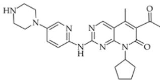
pyridopyrimidine derivative PD 0332991
