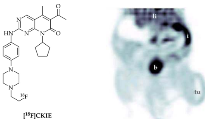
Fig. 3. PET studies with fluorine-18 radiolabeled pyrido[2,3- d ]pyrimidine derivative CKIE
