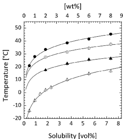
Fig. 2. Observed solubility lines of C 24 , C 28 , C 32 and C 36 waxes (from bottom to top) in decane (Ashbaugh et al., 2002).
