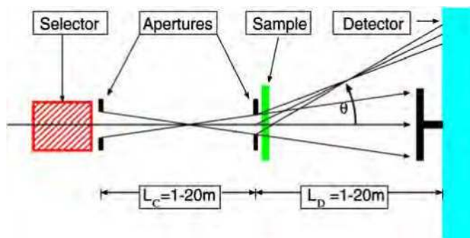
Fig. 6. Principle of pinhole SANS; a neutron beam entering the instrument from the left is the subject of monochromatization (done by the velocity selector), collimation over a variable distance (achieved by using a set of adaptive system of apertures), scattering on the sample and detection on a two-dimensional position sensitive detector over long distances; aiming for detecting neutrons at small scattering angles the SANS instruments are very long.
