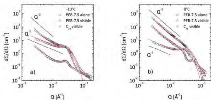
Fig. 14. Examples of wax and polymer SANS profiles (triangles) from PEB- n /wax mixed solutions in decane (Radulescu et al., 2004) for 0.6%PEB-7.5/1%C 24 at -10°C (a) and 0.6%PEB-7.5/0.5%C 36 at 0°C (b); the polymer self-assembling SANS patterns (circles) are shown in parallel in order to emphasize the structural changes induced by the addition of wax; the curves represent model description of the data (see text).
