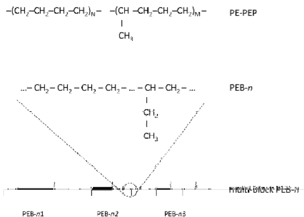
Fig. 4. Polymer structures designed and synthesized as efficient wax crystal modifiers following microstructural studies with SANS: crystalline-amorphous PE-PEP diblocks, semicrystalline PEB- n random copolymers with tuned crystallinity (variable number of ethyl side-groups) and multi-block PEB- n copolymers with graded crystallinity.
