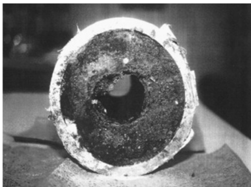
Fig. 3. Plugged pipeline (Banki et al., 2008).
