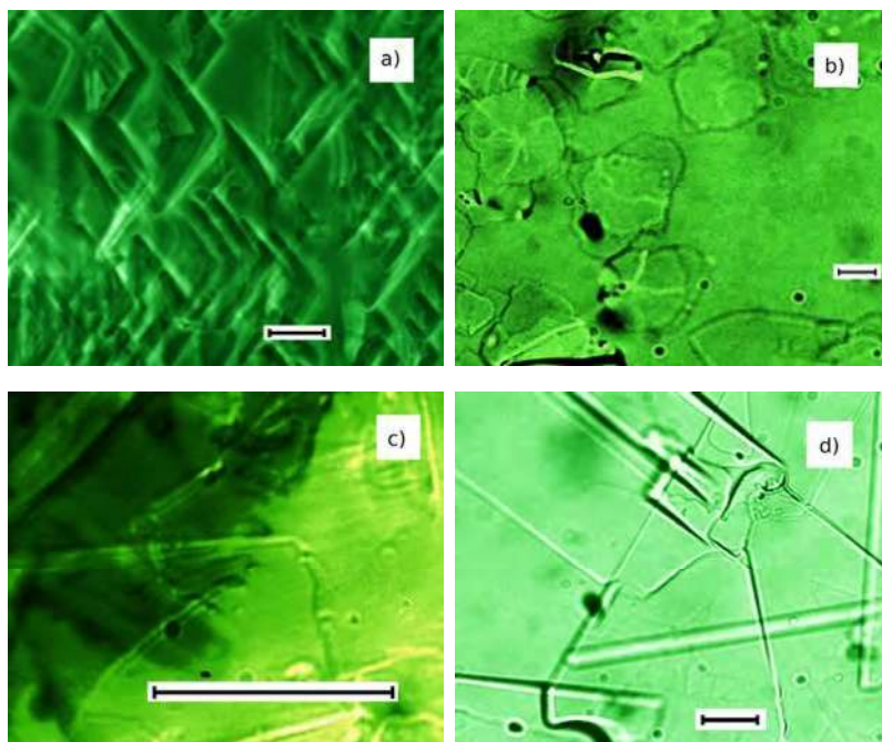
Fig. 8. Micrographs from decane solutions of mixed 1% C_{36} /1% C_{30} at 0°C (a), 0.5% C_{24} at -20°C (b), 1% C_{36} at 20°C (c) and 4% C_{24} at -10°C (d); scale bars 30µm.
