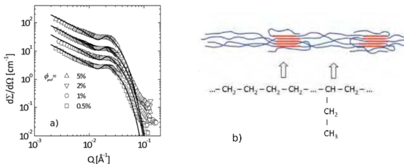
Fig. 12. (a) Examples of SANS patterns from PEB-7.5 copolymer in decane for different \phi_{pol} at -10^{\circ}\text{C} (Radulescu et al., 2004); (b) Sketch depicting the structure of PEB- n random copolymers in solution as emerged from the analysis of SANS data.
