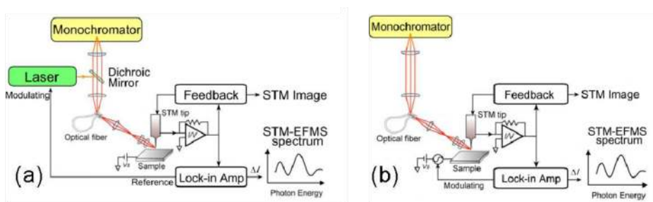
Fig. 4. Schematic illustrations of STM-EFMS measurement: (a) OM scheme, (b) BM scheme. [15]*
