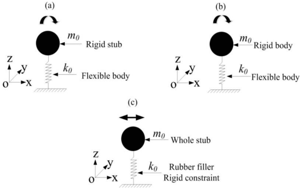
Figure 13. The equivalent theoretical model of the resonator for formation mechanism of the in-plane bandgap of (a) the “transition” PC plate, (b) the classical PC plate, and (c) the broad complete bandgap metal-matrix embedded phononic crystals.
