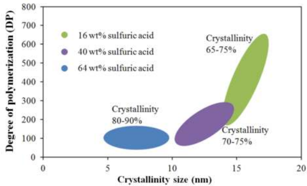
Figure 6. Crystallinity size in relation to the DP. During acid hydrolysis, the DP will decrease and the cellulose crystallinity will increase, due to loss of non-crystalline regions and, as a result, smaller crystal size will be obtained.
