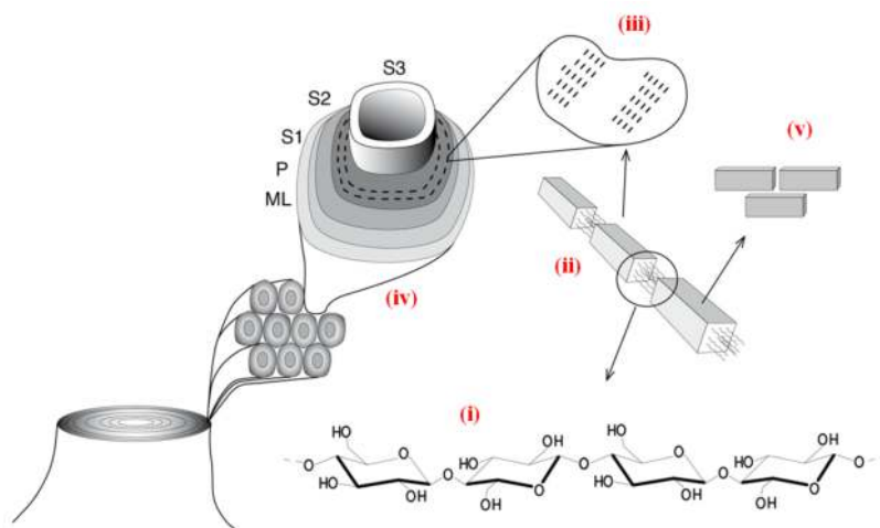
Figure 2. The different levels of the cellulose structure: (i) the molecular structure of a cellulose polymer, (ii) the polymers ordered into microfibrils with crystalline and non-crystalline regions, (iii) several microfibrils assembled together to form a macrofibril, and (iv) the different layers in the cell wall. Numbers (ii) and (v) show cellulose microfibrils (CMFs) and cellulose nanocrystals (CNCs), respectively. Illustration: Jari Sundqvist.
