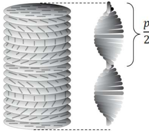
Figure 4. At certain concentrations, the nanocrystals self-organize into a chiral nematic ordering where the length of the pitch gap ( p ) in the helical structure can absorb different wavelengths and emit wavelengths with different colors. Illustration: Jari Sundqvist.
