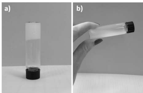
Figure 8. Thixotropic behavior of the fully dried CNC sample re-dispersed in water to a CNC concentration of 4.15%. (a) In static mode and (b) immediately after agitation.
