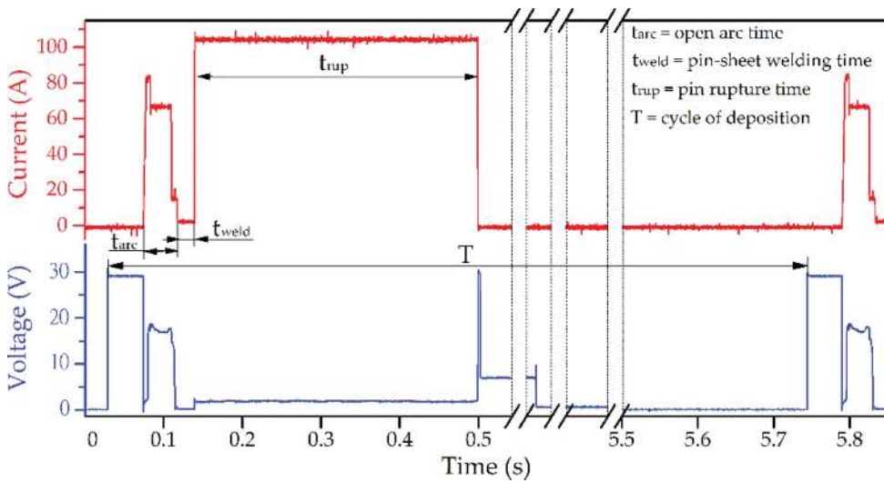
Figure 2. Cycle of pin deposition based on the electrical current and voltage data.
