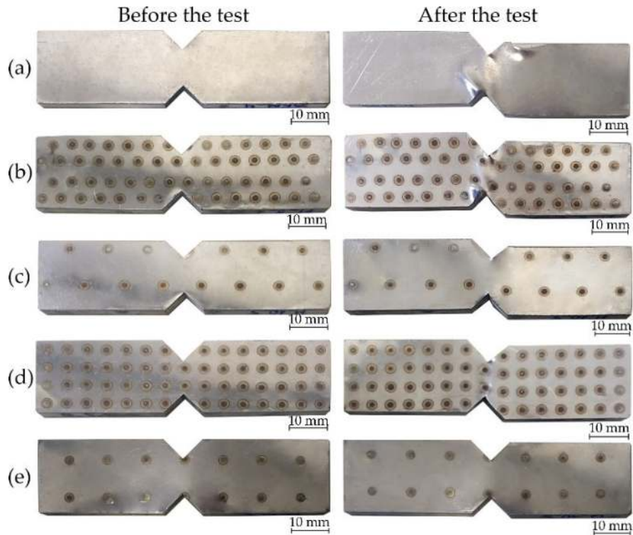
Figure 24. Typical aspect of the five types of FMLP's specimens before (left) and after (right) the Iosipescu shear test, where: (a) M-C-M (without pins); (b) MPin-C-MPin hexagonal 5; (c) MPin-C-MPin hexagonal 10; (d) MPin-C-MPin squared 5; (e) MPin-C-MPin squared 10.
