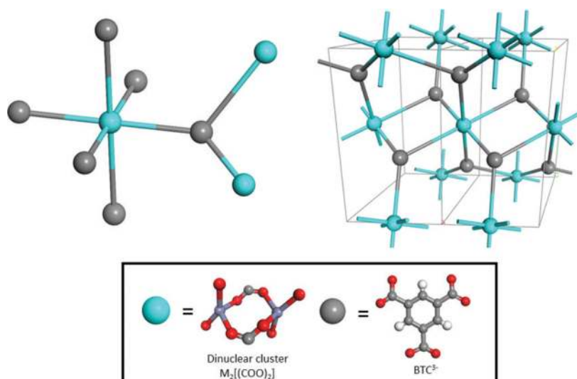
Figure 7. The structure represents (3,6)-connected network. This corresponds to the following formulas: [BMI][Zn(BTC)] (FÜTZEB), and [EMI] 2 [In 2 Co(OH) 2 (BTC) 2 Br 2 ] (VUVZAP).
