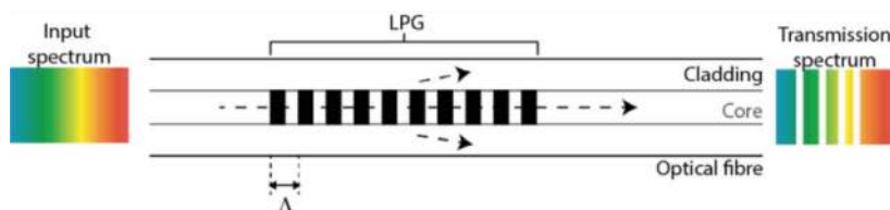
Figure 1. Schematic diagram of an LPG.
