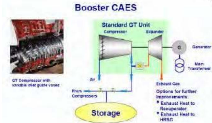
Fig. 9. Air Injection (AI) or booster CAES (Alstom Power)
