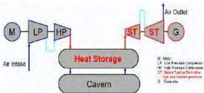
Fig. 11. Advanced Adiabatic CAES Concept (Alstom Power)
