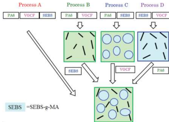
Figure 17. Schematic diagram of four different processing sequences for ternary composites (VGCF/PA6/SEBS-g-MA).
