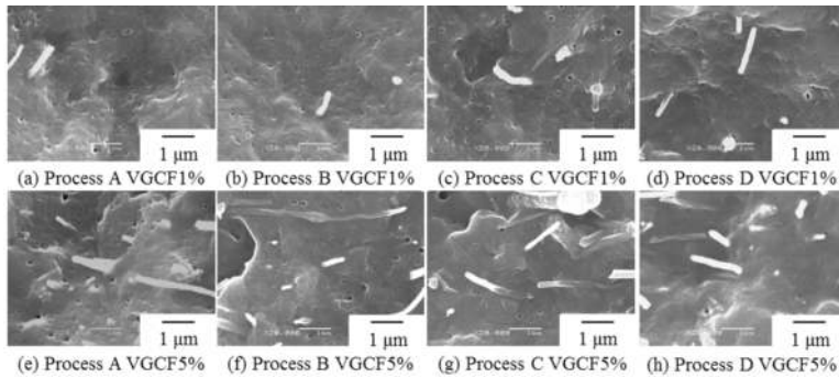
Figure 20. SEM micrographs of etched fracture surface for various processing sequence of the ternary composites (VGCF/PA6/SEBS-g-MA) (SEBS-g-MA content is 20 wt% and etched with toluene for 24 h to remove the dispersed phases): (a) Process A VGCF 1%, (b) Process B VGCF 1%, (c) Process C VGCF 1%, (d) Process D VGCF 1%, (e) Process A VGCF 5%, (f) Process B VGCF 5%, (g) Process C VGCF 5%, and (h) Process D VGCF 5%.
