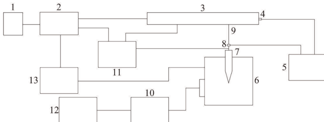
Figure 3. Schematic diagram of the high-pressure common rail fuel injection system test bench. 1. Drive motor 2. High pressure fuel pump 3. Common rail 4. Common rail pressure sensor 5. Oscilloscope 6. Mechanical part of IFR 7. Injector 8. Pressure sensor 9. High pressure pipeline 10. Electronic part of IFR 11. ECU 12. Computer terminal 13. Tank.
