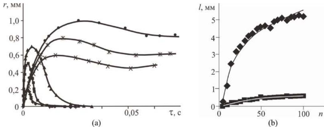
Figure 7. Changes in border radius zone temperature field ( T = 850^\circ\text{C} ) as a function of time for different processing methods LC ( \times , \mathcal{K} , \bullet ), LCC ( \blacktriangle ), WJGL ( \blacklozenge , \blacksquare ) (a) and cutting depth in materials (HA, \blacklozenge ; PSTM, \blacksquare ) depending on the number of cuts (b).
