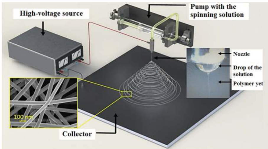
Figure 2. A diagram of a stand for the production of nanofibers containing a picture showing the mouth of the nozzle and a drop of the polymer solution that forms under the influence of high voltage in the so-called Taylor cone from the apex, which is followed by a shot of a thin stream of the solution.
