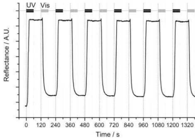
Figure 4. Time-dependent change in the reflectance of 5CB/azobenzene LC mixture-infiltrated inverse opal film at 603 nm by UV and visible light irradiation. The black bars show the periods for the irradiation of UV light (<math><400\text{ nm}</math>), and the gray bars show the periods for irradiation of visible light (436 nm). For other periods, the sample was kept in the dark [58]. Copyright 2002, American Chemical Society.
