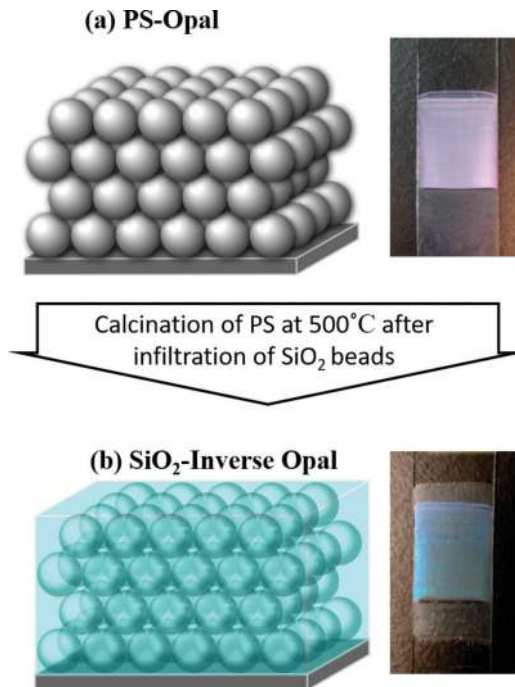
Figure 2. Schematic of PS opal (a) and \text{SiO}_2 inverse opal (b) structures and their photographs.
