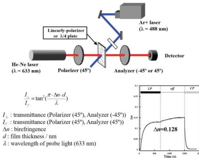
Figure 7. Schematic for birefringence measurement and the result of PAz.
