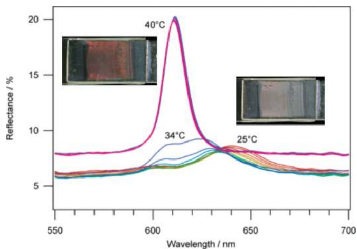
Figure 3. Reflection spectra of \text{SiO}_2 inverse opal film infiltrated with 5CB at the temperature from 25°C to 40°C [50]. Reproduced. Copyright 2004, American Chemical Society.
