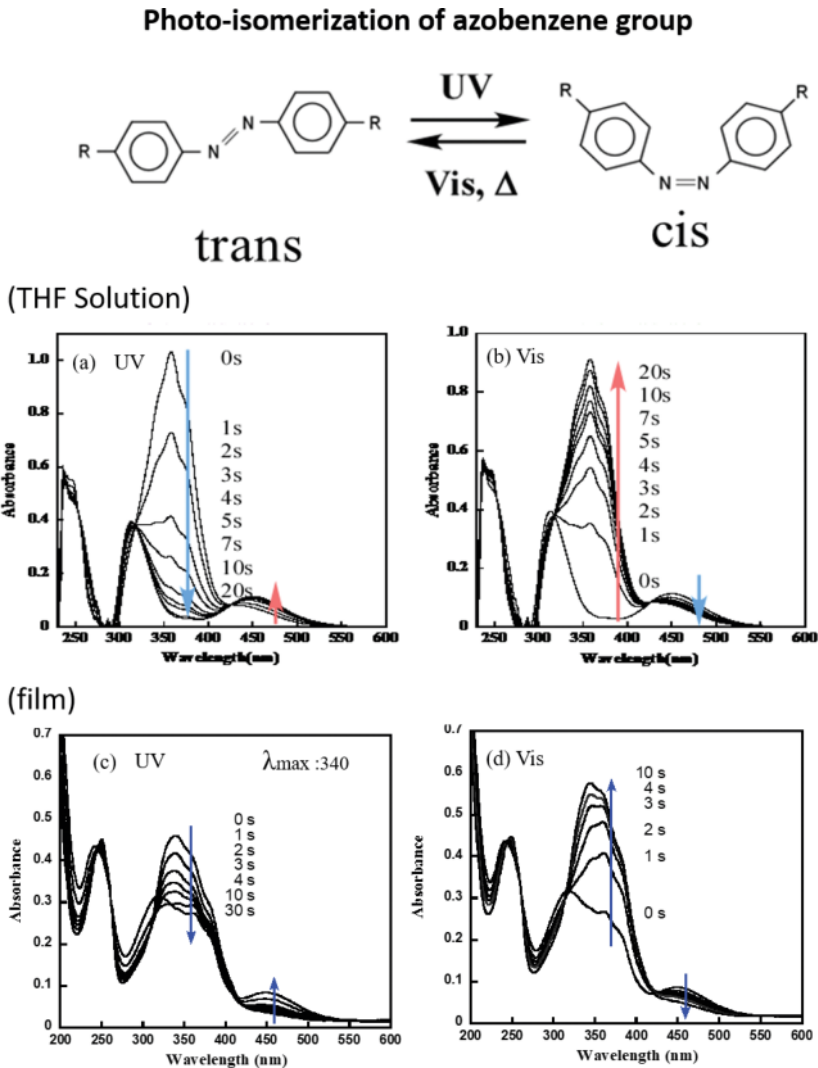
Figure 6. Changes in absorption spectra of PAz in THF after UV light (365 nm, 8 mW/cm 2 ) (a) and visible light (436 nm, 60 mW/cm 2 ) (b) irradiation. Changes in absorption spectra of PAz film irradiated UV light (365 nm, 10 mW/cm 2 ) (c) and following visible light (436 nm, 58 mW/cm 2 ) (d) at room temperature.
