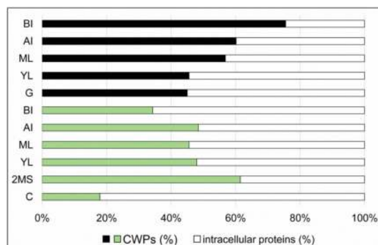
Figure 2. Percentage of CWPs and proteins predicted to be intracellular in each proteome. B. distachyon proteomes are in black and white, whereas sugarcane proteomes are in green and white. AI: apical internodes; BI: basal internodes; C: cell suspension cultures; G: grains; ML: mature leaves; YL: young leaves; 2MS: 2-month-old stems.
