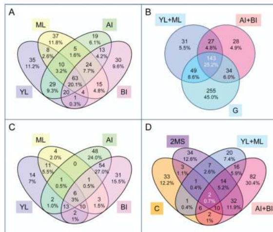
Figure 3. Venn diagrams showing common and specific CWP's for each experiment performed with B. distachyon (A and B) or sugarcane (C and D). AI: apical internodes; BI: basal internodes; C: cell suspension cultures; G: grains; ML: mature leaves; YL: young leaves; 2MS: 2-month-old stems.
