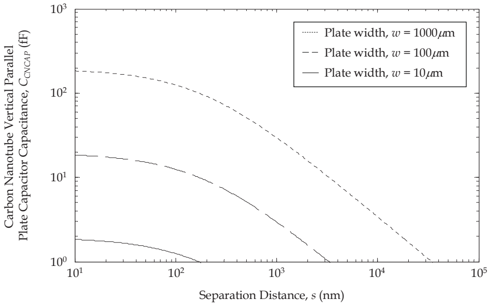
Fig. 9. Carbon nanotube vertical parallel plate capacitor capacitance, C_{CNCAp} , vs. plate separation distance, s , and plate width, w .
