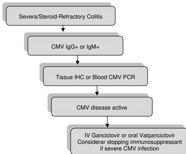
Figure 3. Algorithm for management of suspected CMV colitis in patients with IBD [4]
