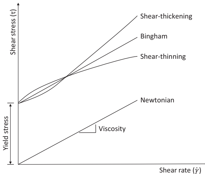
Figure 2.2 Shear curves different materials.
