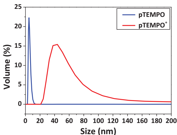
Figure 4.8 Dynamic light scattering measurements of pTEMPO; poly(MAA-co-TEMPO) and pTEMPO + ; poly(MAA-co-TEMPO + ) at a polymer concentration of 5 mg/ml in cement pore solution.
