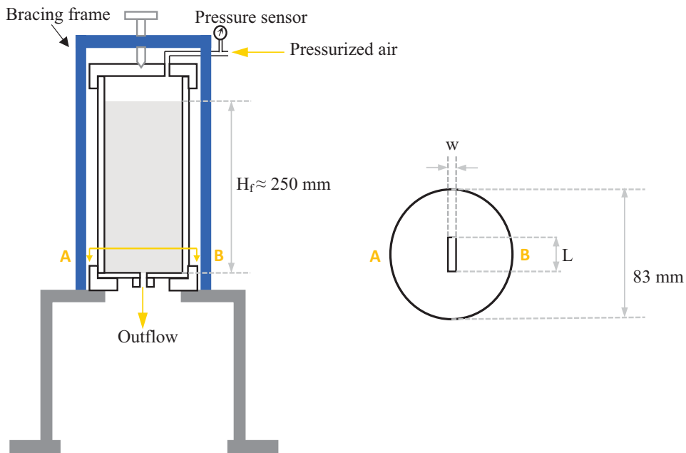
Figure 6.4 Experimental set-up for the study of leakage.
