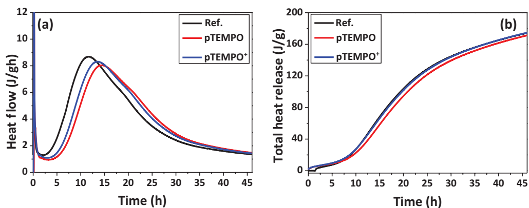
Figure 4.9 Time-dependent heat flow (a) and total heat (b) liberated by cement pastes ( W/C = 0.4 ) at a temperature of 20\text{ }^{\circ}\text{C} in the presence of 0.1% bwoc of pTEMPO; poly(MAA-co-TEMPO) and pTEMPO + ; poly(MAA-co-TEMPO + ) copolymers and compared to reference cement paste, as determined by isothermal calorimetry.
