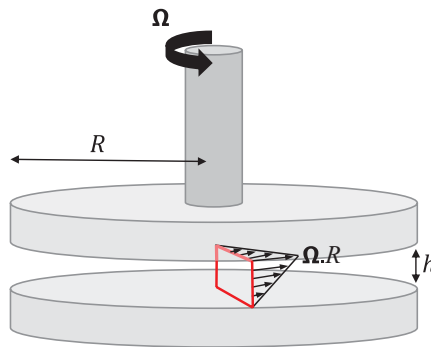
Figure 2.3 Parallel plate geometry schematically. Source: after [7].
