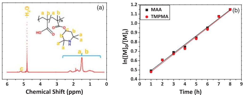
Figure 4.3 1 H-NMR spectra of purified poly(MAA-co-TMPMA) in D 2 O (a) and first order kinetic plot for the synthesis of PCA by copolymerization of MAA and TMPMA; [MAA]:[TMPMA]:[CTA]:[AIBN] = 50:50:1:0.2, [M] = 1 M in EtOH/H 2 O (80/20) at 70 °C (b).
