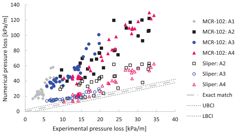
Figure 8.8 Comparison of numerically simulated pressure loss with experimentally obtained pumping results, for four different mixture designs (A1 to A4), based on rheological input from the MCR-102 rheometer and the Sliper. Pressure sensor uncertainty is indicated by the upper and lower boundary (UB and LB) confidence intervals (CI). Source: adapted from [48].
