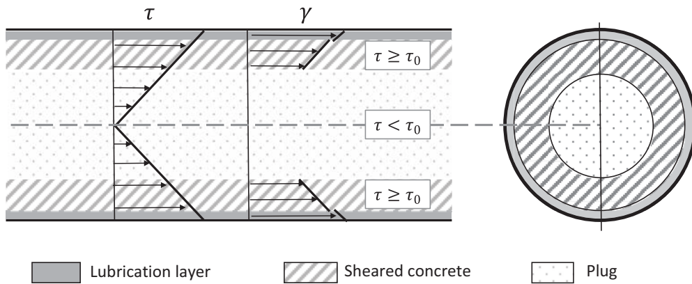
Figure 2.16 Flow profile in a pipe. Source: after [63].
