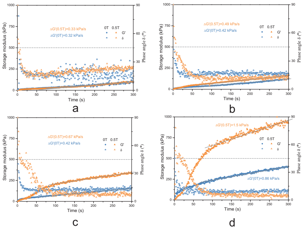
Figure 3.17 Influence of particle concentration on the early structural evolution of cementitious paste ( w/c=0.4 and nano-Fe 3 O 4 of 20–30 nm). (a) 0% nano-Fe 3 O 4 ; (b) 0.25% nano-Fe 3 O 4 ; (c) 1% nano-Fe 3 O 4 and (d) 3% nano-Fe 3 O 4 . \Delta G' is the increase rate of storage modulus at steady state. Source: after [63].
