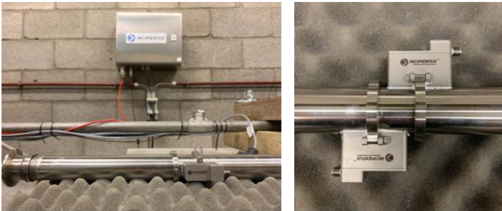
Figure 5.5 Illustration of equipped ultrasonic velocity profiler. (Left) Pipe section on which acoustic transducers are mounted under an inclined angle. (Right) Close-up of acoustic transducers by which ultrasound pulses travel from one sensor to another and back. Source: originating from [6].
