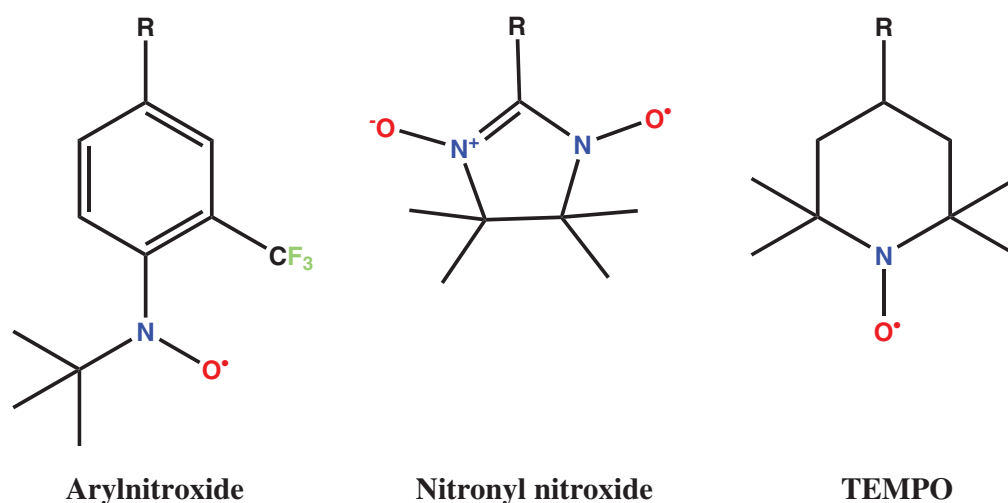
Figure 4.1 Some examples of common nitroxide radicals.
