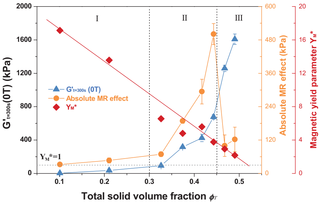
Figure 3.14 Correlations between G'_{t=300s}(0T) , difference of G'_{t=300s} , and magnetic yield parameter for cementitious pastes with fixed nano- Fe_3O_4 (100 nm) concentration of 3% by mass of cement + water. \phi_T is the total solid volume fraction. Error bar indicates the standard deviation. Source: after [70].
