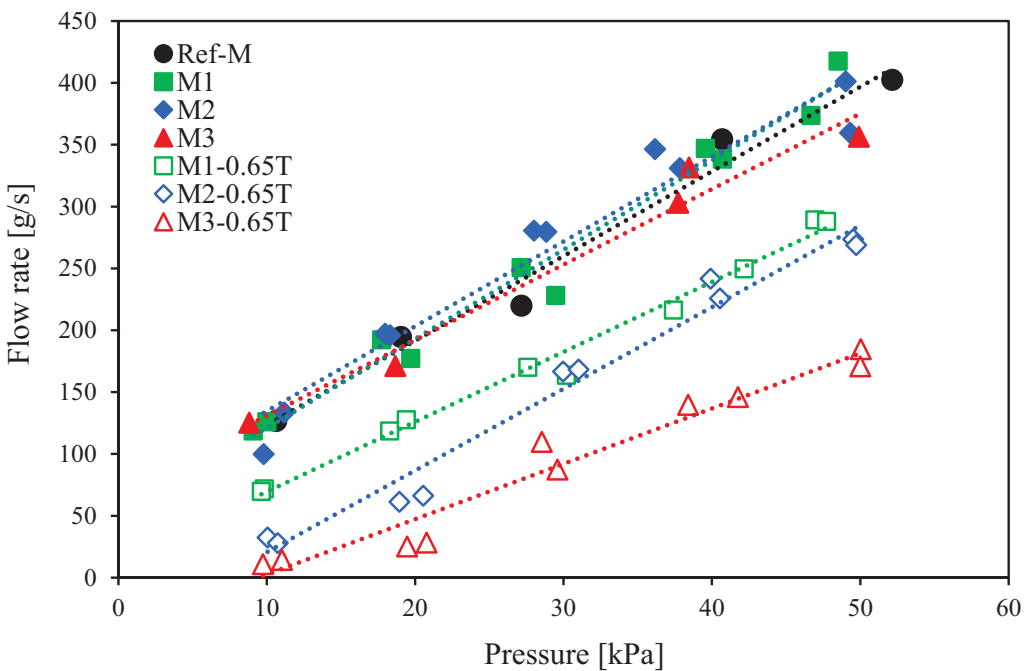
Figure 6.18 Effect of MNP concentration on initial mass flow rate – medium slump paste.
