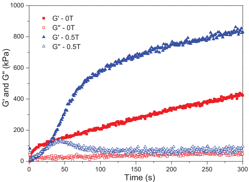
Figure 3.11 Evolution of storage modulus and loss modulus for cementitious paste with w/c of 0.4 and nano- \text{Fe}_3\text{O}_4 (20–30 nm) content of 3%, in the absence and presence of magnetic field of 0.5 T. Source: after [36].
