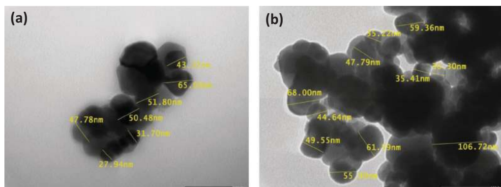
Figure 4.14 TEM images of (a) bare Fe 3 O 4 NPs and (b) polyDopmaMA-coated Fe 3 O 4 NPs.
