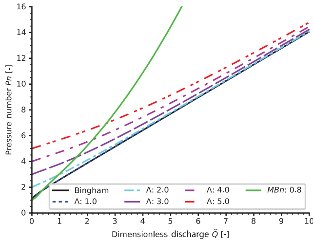
Figure 5.2 Non-dimensional discharge diagram for a spectrum of material parameters of cementitious suspensions, based on Poiseuille flow extensions (i.e. Bingham, modified Bingham and simplified Rousel). Source: after [6, 11].
