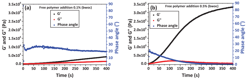
Figure 4.23 Results of time sweep measurements of cement pastes containing free poly(MAA-co-PEGMA 500 -co-DopaMA) terpolymer at a concentration of (a) 0.1% bwoc and (b) 0.5% bwoc at w/c = 0.45; all DopaMA-based terpolymers show a similar trend.
