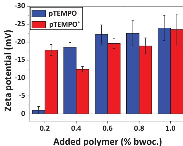
Figure 4.7 Zeta potential measurements of cement particles in the presence of poly(MAA-co-TEMPO) copolymers at different polymer concentrations (% bwoc) at W/C= 50; the average of five measurements was represented; pTEMPO = poly(MAA-co-TEMPO) and pTEMPO + =poly(MAA-co-TEMPO + ).
