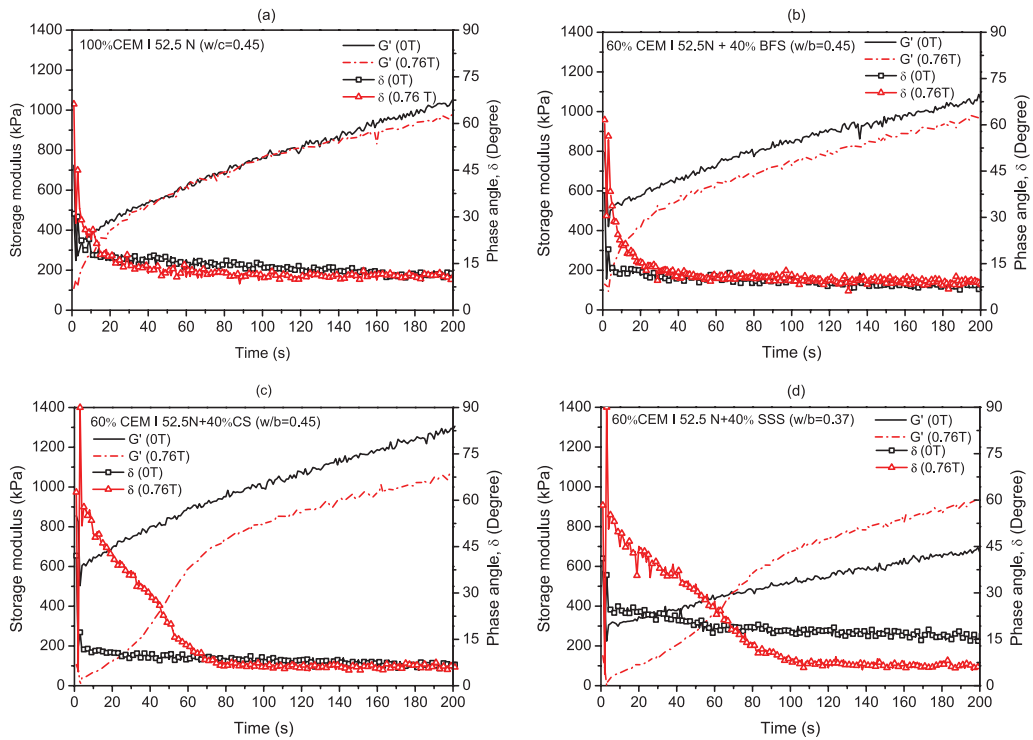
Figure 3.3 Storage modulus and phase angle evolution of Portland cement paste (a), blast furnace slag (b), copper slag (c) and stainless steel slag (d) incorporated pastes without (0 T) and with magnetic field of 0.76 T.
