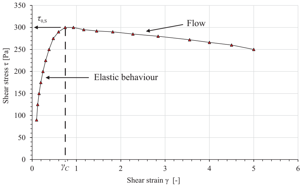
Figure 2.7 Stress–strain diagram with peak value. Source: after [7].
