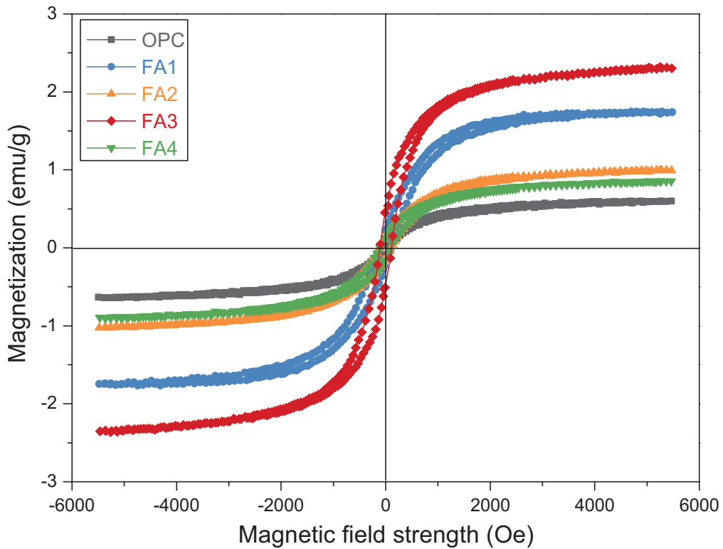
Figure 3.25 Magnetization loop curves of representative fly ashes. Source: after [96].
