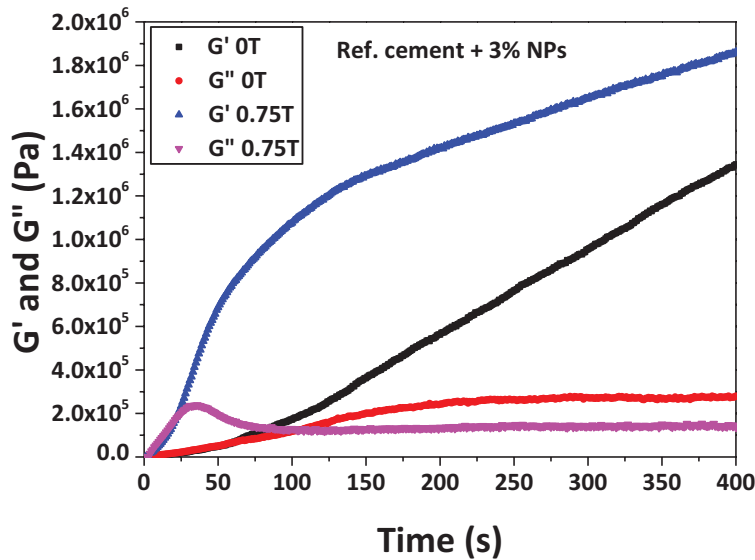
Figure 4.21 Results of time sweep measurements of cement pastes containing \text{Fe}_3\text{O}_4 NPs at W/C = 0.45 ; magnetic field strengths ( B ) of 0 T and 0.75 T have been applied.
