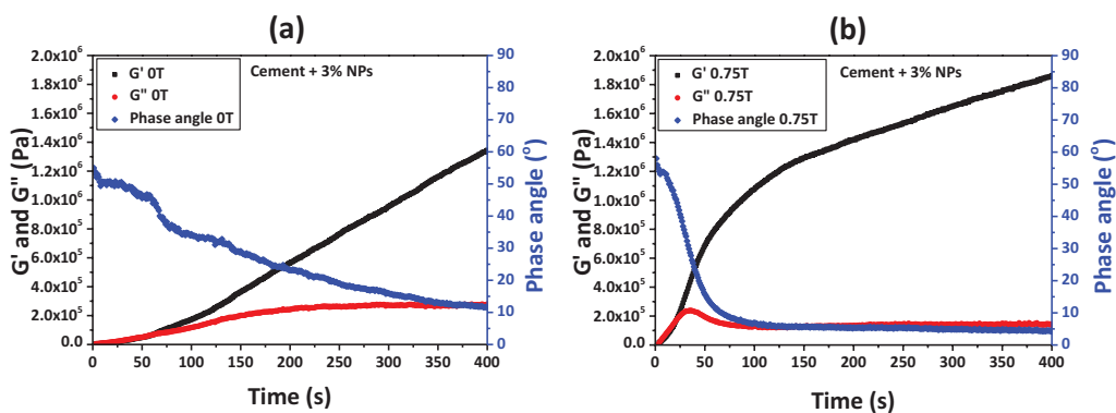
Figure 4.22 Results of time sweep measurements of cement pastes containing \text{Fe}_3\text{O}_4 NPs at W/C = 0.45 ; magnetic field strengths ( B ) of 0 T and 0.75 T have been applied.
