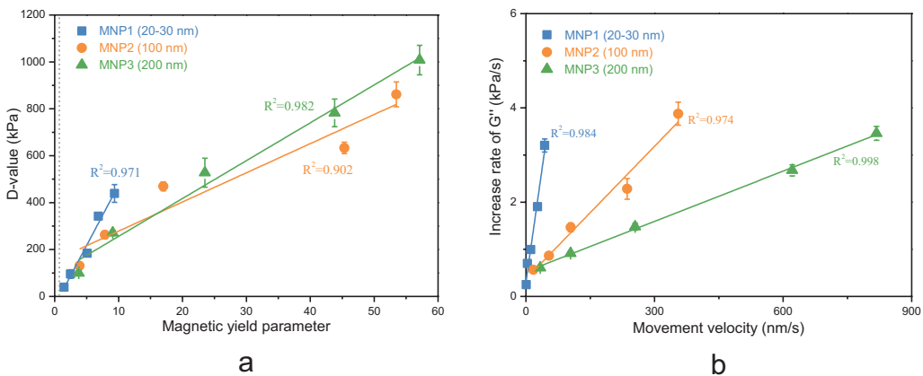
Figure 3.21 Relationship between measured magneto-rheological properties and calculated theoretical parameters. (a) D -value versus magnetic yield parameter, and (b) early increase rate of loss modulus versus movement velocity of nanoparticles. Error bar indicates the standard deviation. Source: after [63].
