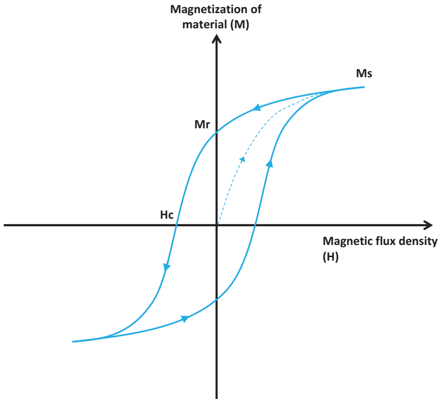
Figure 3.2 Typical magnetization hysteresis curve of a ferromagnetic material. Ms is the maximum magnetization ( \text{Am}^2/\text{g} or \text{emu/g} ), Mr is the magnetization left behind in a material after an external magnetic field is removed ( \text{Am}^2/\text{g} or \text{emu/g} ), and Hc is the ability of a material to withstand a magnetic field without becoming demagnetized (Oe).
