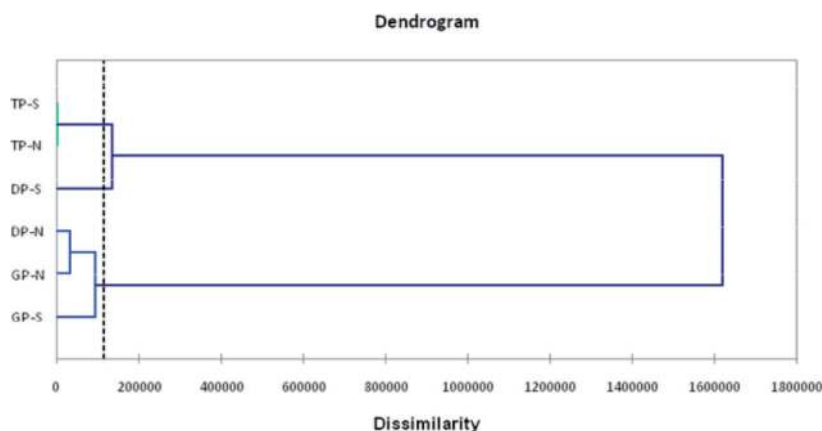
Figure 3. Dendrogram of grouping of sediment sampling stations.
