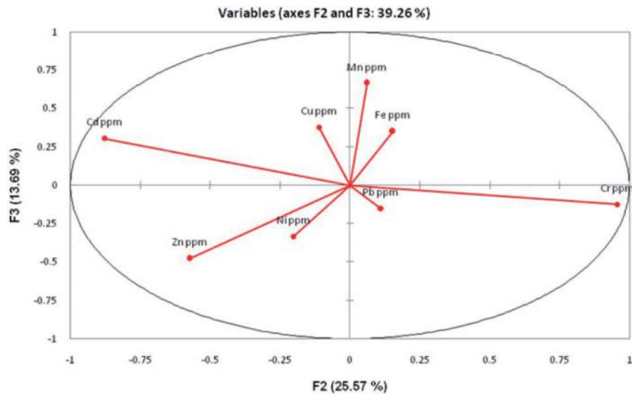
Figure 5. Factors 2 & 3 assemblage of the heavy metals.
