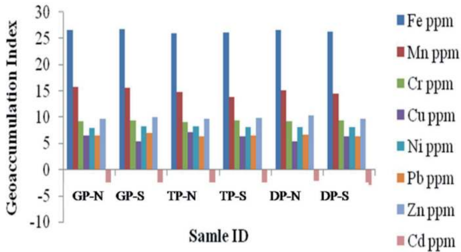
Figure 7. Graphical representation of Igeo for heavy metals.
