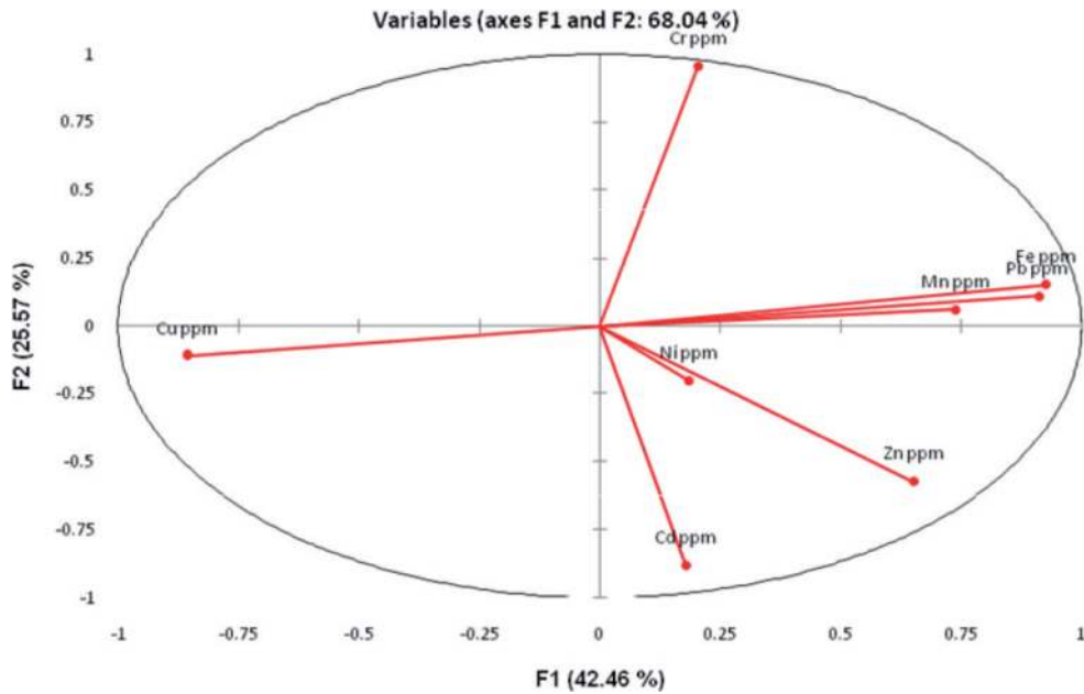
Figure 4. Factors 1 & 2 assemblage of the heavy metals.
