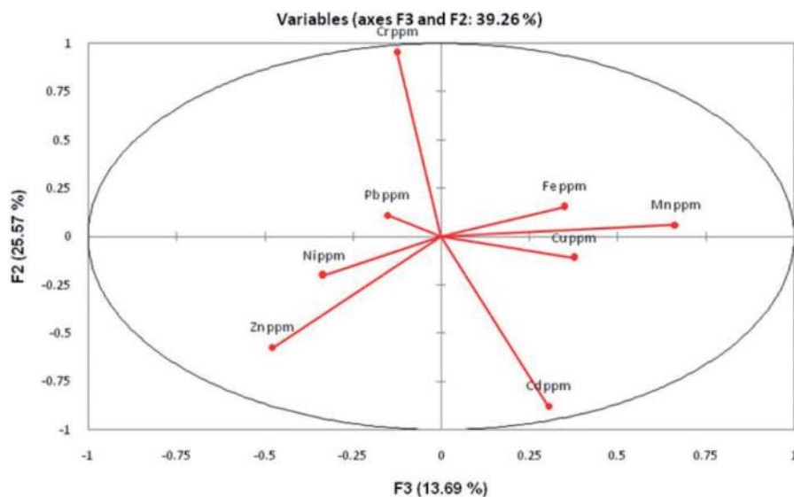
Figure 6. Factors 3 & 2 assemblage of the heavy metals.
