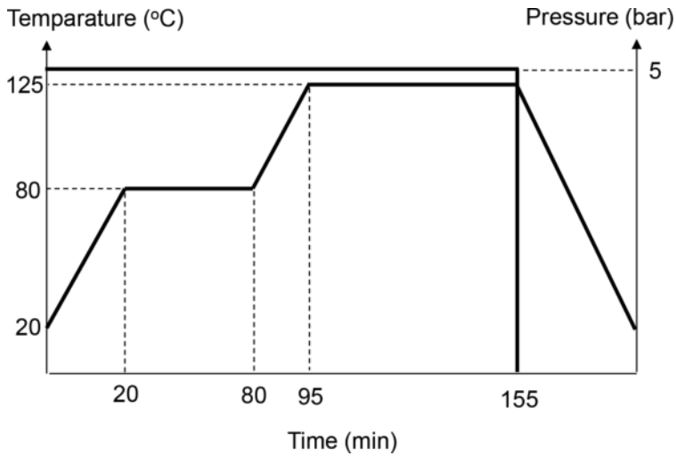
Figure 1. Curing cycle of the composite laminate fabrication.
