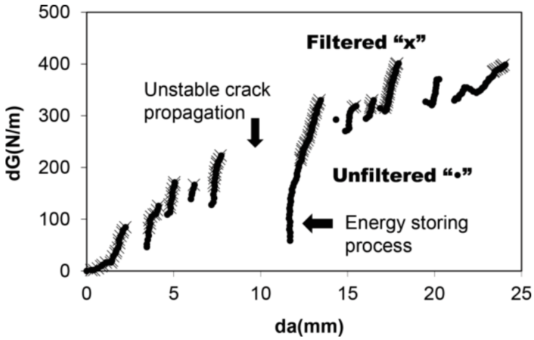
Figure 6. R-curve of the DCB specimens.
