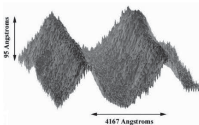
Figure 13. AFM image of 2400/mm replica grating (after [31]).
